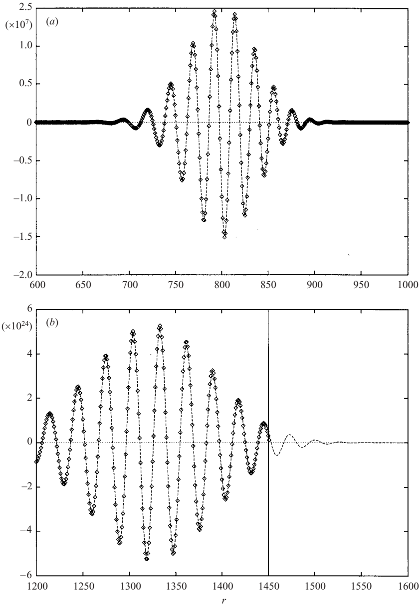
FIGURE 25. Instantaneous radial variation of \omega_{\theta w} for an impulsively excited disturbance with n=67 and r_e=530 . (a) t/T=0.796 ; (b) t/T=1.592 . The computational outflows are again located at r_o=1450 (diamonds) (indicated in (b) by a vertical line): r_o=1700 (dashed lines).
