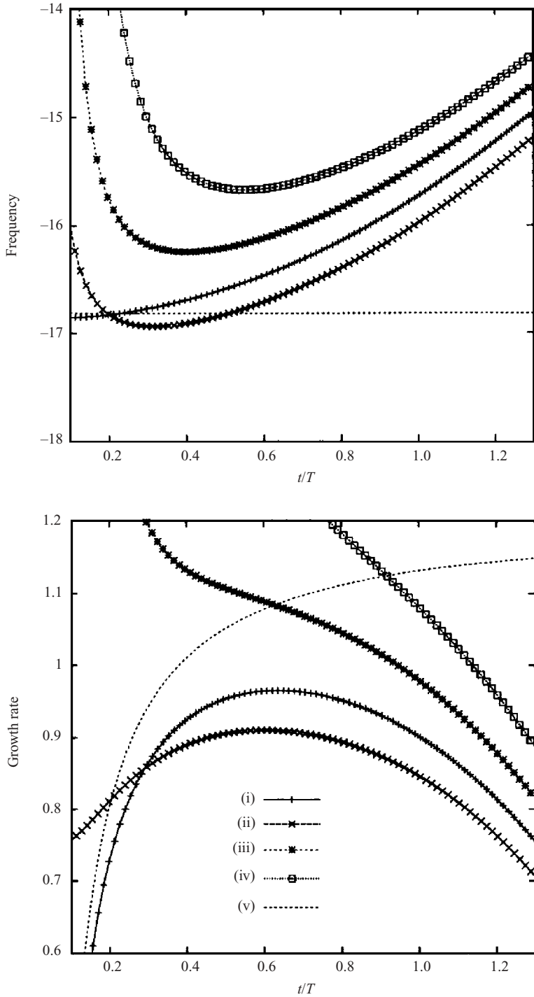
FIGURE 18. Local temporal frequencies \bar{\beta}_r R and temporal growth rates \bar{\beta}_i R for a disturbance with n = 75 . For the curves labelled (i)–(iv) the impulsive excitation was centred at r_e = 650 and the flow is spatially inhomogeneous. The temporal development is plotted for the radial positions: (i) r = r_e = 650 ; (ii) r = 625 ; (iii) r = 675 ; (iv) r = 700 . The curves labelled (v) show the development at the point of impulsive excitation of a similar disturbance in a spatially homogeneous flow with R = 650 .
