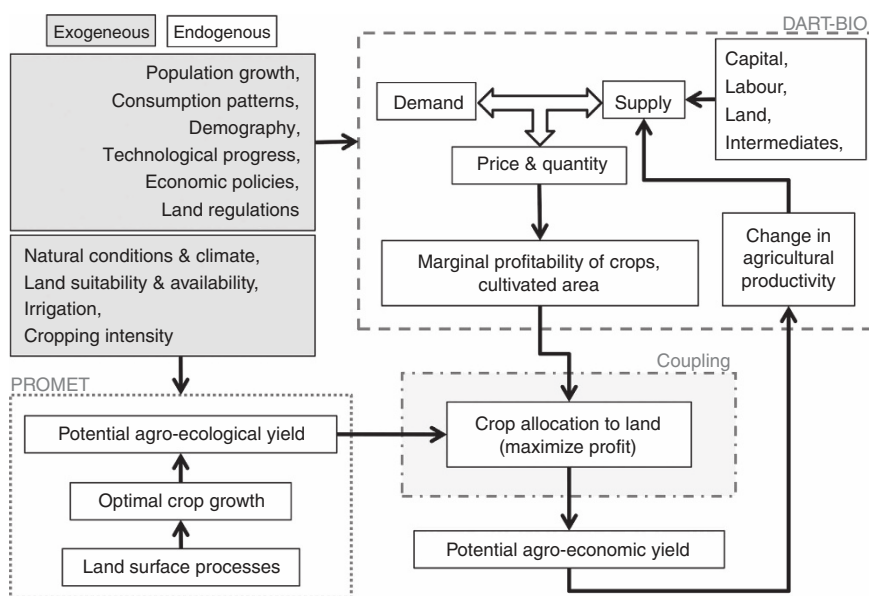
Figure 5 | Conceptual framework for the coupled simulation of regional and global agro-economic potential biomass production increase (PBPI). The simulations of potential agro-ecological yields from PROMET (lower left) and marginal profitability resulting from balancing demand and supply in DART-BIO (upper right) are coupled (centre) to determine profit-maximizing crop allocations to land, which result in potential agro-economic yields. The exogenous inputs to DART-BIO and PROMET are listed in the in the upper left boxes.
