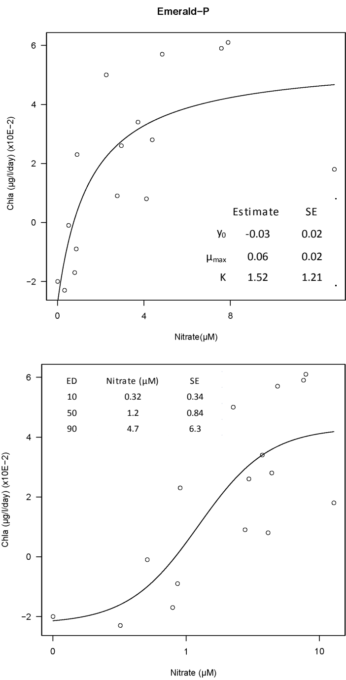
Figure 4.15: Monod (top) and dose response (bottom) curves for the Emerald-P cubitainer experiment.
