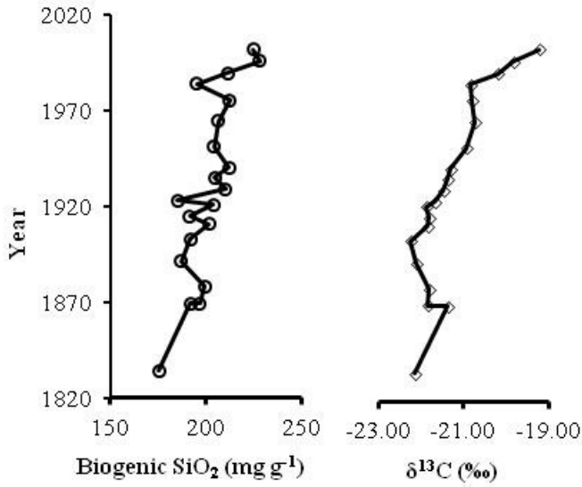
Figure 2.5: BSi and \delta^{13}\text{C} profiles for Moat Lake.
