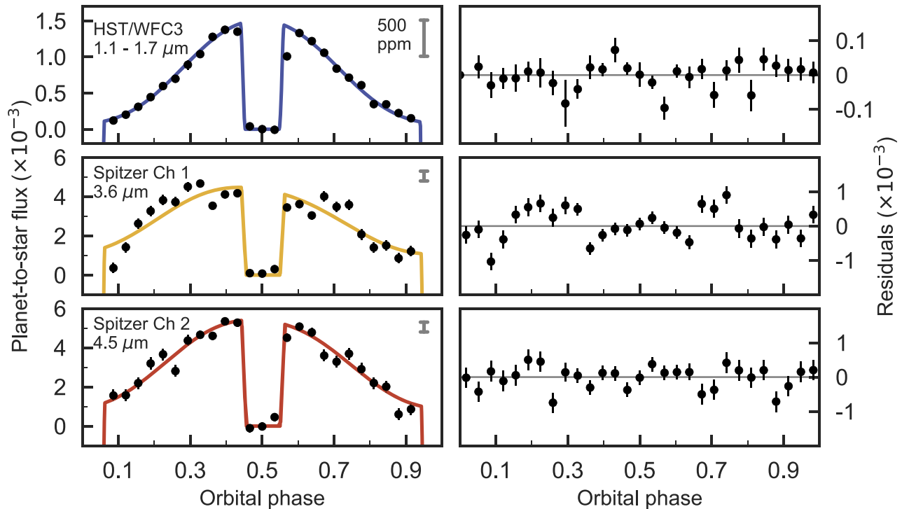
Figure 5. WASP-103b phase curve observations from HST /WFC3 (top) and Spitzer /IRAC (middle and bottom). For clarity, the data are phase-folded on the planet’s orbital period and binned in 30 uniformly spaced bins between 0 and 1 (corresponding to 0.8 hr). The left column shows the phase curves with systematic noise removed (black points) compared to the best-fit spherical harmonics model (colored lines). The error bars denote 1\sigma uncertainties (in some cases, the errors are smaller than the data points). We include the transits in the fit, but they are not displayed in this figure. The right-hand column shows the binned residuals for the best-fit light curve. The gray error bars in the upper right of the left panels correspond to 500 ppm, to illustrate the changing y-axis scale.
