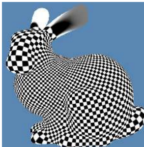
(b) The global parameterization induced from (a)
