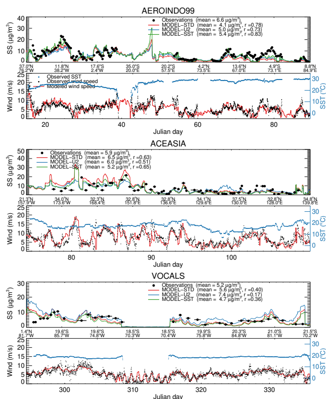
Fig. 3b. Same as Fig. 3a but for the AEROINDO99, ACE-ASIA, and VOCALS PMEL cruises.
