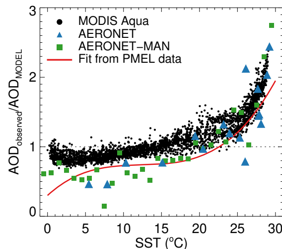
Fig. 10. SST dependence of the ratio of annual mean MODIS Aqua to MODEL-STD AOD. We only show points for regions where u_{10m} > 6\text{ m s}^{-1} and modeled SS account for more than 60% of the total modeled AOD. The blue triangles correspond to the annual mean ratio of the 17 AERONET sites displayed in Fig. 11. The green squares are for the Maritime Aerosol Network (AERONET-MAN) binned by SST. The red line is the polynomial fit obtained from least-squares fitting of C_{\text{obs}}/C_{\text{model}} in Fig. 6.
