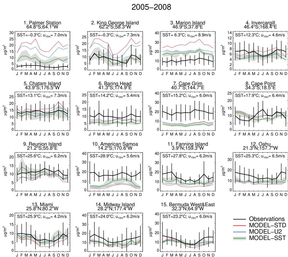
Fig. 7. SS mass concentrations measurements at 15 U. Miami ground-based stations. The locations of the stations are indicated in Fig. 1a. The observations are shown with black lines and error bars corresponding to the standard deviation of the multi-year mean. Three model simulations are shown (MODEL-STD in red, MODEL-U2 in blue, and MODEL-SST in green), with the seasonal variations calculated from 2005–2008 monthly means. For MODEL-SST the grey area indicates the interannual variability for these four years. The annual mean u_{10\text{m}} and SST are listed in each panel. When the stations are located in regions surrounded by sea ice (Palmer Station and King George Island) we use the SST of the closest ice-free region.
