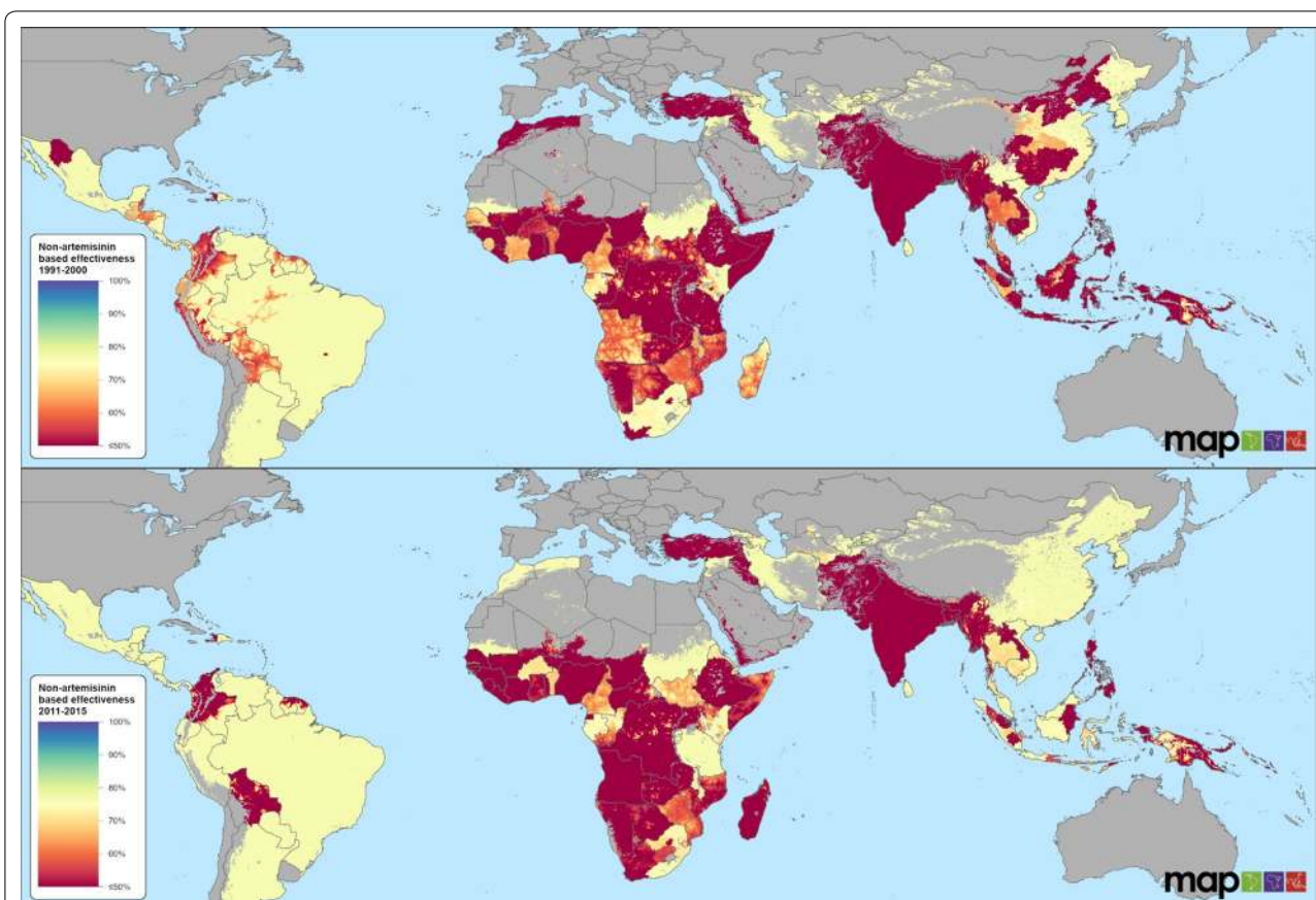
Fig. 2 Spatiotemporal distribution of effectiveness of non-artemisinin anti-malarial drugs for periods 1991–2000 and 2011–2015. Maps for 2001–2005 and 2006–2010 are presented in Additional file 1: Figure S4.2
