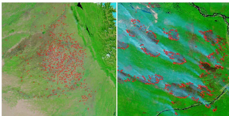
Fig. 1. Aqua MODIS 500-m false color imagery of northern India (left) on 23 October 2004 (08:20 UTC) and Yakutsk, Russia (right) on 19 August 2002 (03:00 UTC). Outlines of 1-km active fire pixels are shown in red. With this band combination ( 2.1 \mu\text{m} , near-infrared, red) dense vegetation appears green, heavy smoke appears light blue, burn scars appear dark brown, water appears black, and non-cirrus clouds appear white. The scale (approximately 320 \times 320 \text{ km} ) is identical in both images. Note how larger Yakutsk burn scars are accompanied by large clusters of adjacent fire pixels, while the small (but numerous) agricultural burns in India are characterized by much smaller clusters of fire pixels and no visible burn scars. Images were produced within the MODIS Rapid Response System and appear courtesy of Jacques Desclotres.
