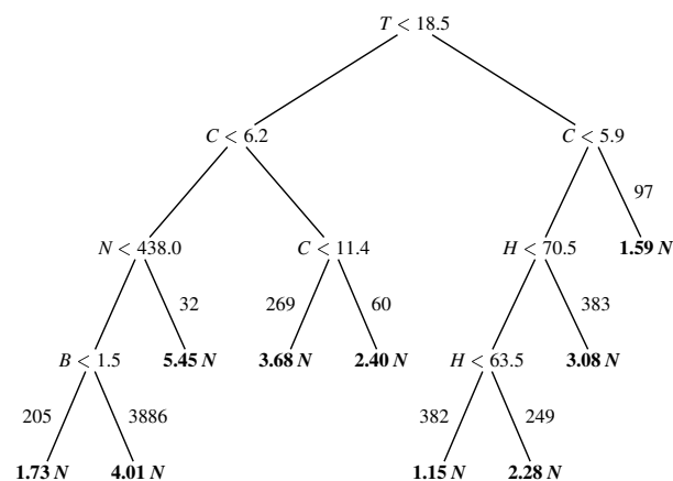
Fig. 9. Same as in Fig. 7 but for Australia.
