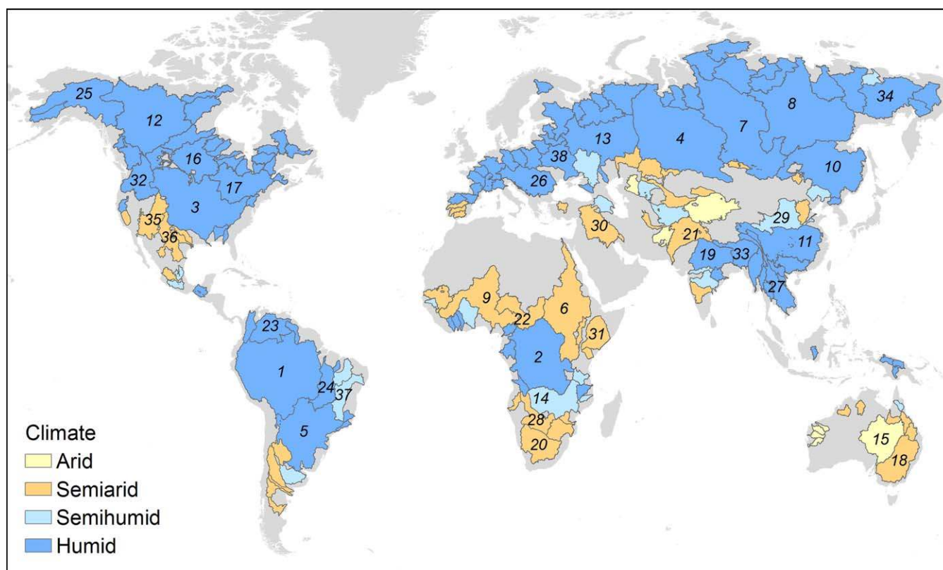
Figure 2. Distribution of river basins (176 total) according to climate. Basins with areas \geq 500,000 \text{ km}^2 are numbered 1 through 38 in order of decreasing basin area. The climate categories include hyperarid and arid (AI: 0.0–0.2, 8 basins), semiarid (AI: 0.2–0.5, 46 basins), subhumid (AI: 0.5–0.65, 19 basins), and humid (AI: > 0.65 , 103 basins). The numbered river basins include 1, Amazon; 2, Congo; 3, Mississippi; 4, Ob; 5, Parana; 6, Nile; 7, Yenisei; 8, Lena; 9, Niger; 10, Amur; 11, Yangtze; 12, MacKenzie; 13, Volga; 14, Zambezi; 15, Lake Eyre; 16, Nelson; 17, St. Lawrence; 18, Murray; 19, Ganges; 20, Orange; 21, Indus; 22, Chari; 23, Orinoco; 24, Tocantins; 25, Yukon; 26, Danube; 27, Mekong; 28, Okavango; 29, Huanghe (Yellow River); 30, Euphrates; 31, Jubba; 32, Columbia; 33, Brahmaputra; 34, Kolyma; 35, Colorado; 36, Rio Grande; 37, Sao Francisco; and 38, Dnieper. Basin areas, climate, and irrigation intensity can be found in Table S1.
