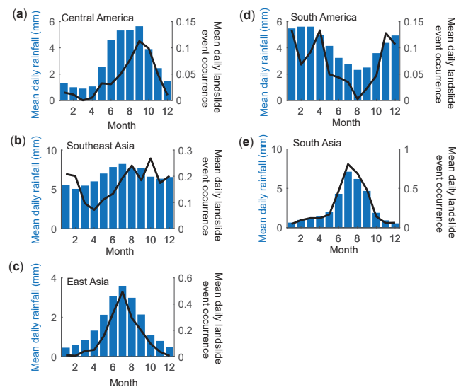
Figure 5. Mean daily rainfall (in millimetres) by month between 2004 and 2016, summarised by geographical subregion (blue bars). Global Precipitation Climatology Centre data (Xie et al., 2013; GPCC, 2018) were processed in ESRI ArcMap and MATLAB. Mean daily rainfall-triggered landslide event occurrence by month between 2004 and 2016 (black line). Daily values are used to overcome the difference in month length.
