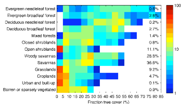
Fig. 2. Percent of burned area within each land cover class (MODIS2Q1, UMD land cover classification) as a function of fractional tree cover (MOD44, 5% bins). Numbers on the right denote the average contribution of each land cover type to global burned area over 2001–2009.
