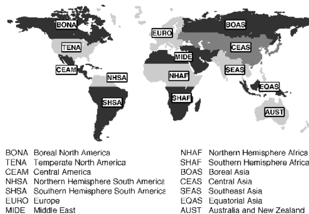
Fig. 7. Map of the 14 regions used in this study, after Giglio et al. (2006) and van der Werf et al. (2006).
