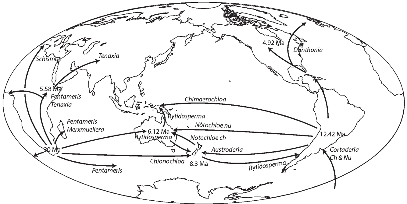
Fig. 3. Biogeographical history of Danthonioidae, showing the inferred dispersal routes, and the dated median age of the first radiations on each continent. Modified from Linder et al. (2013).
