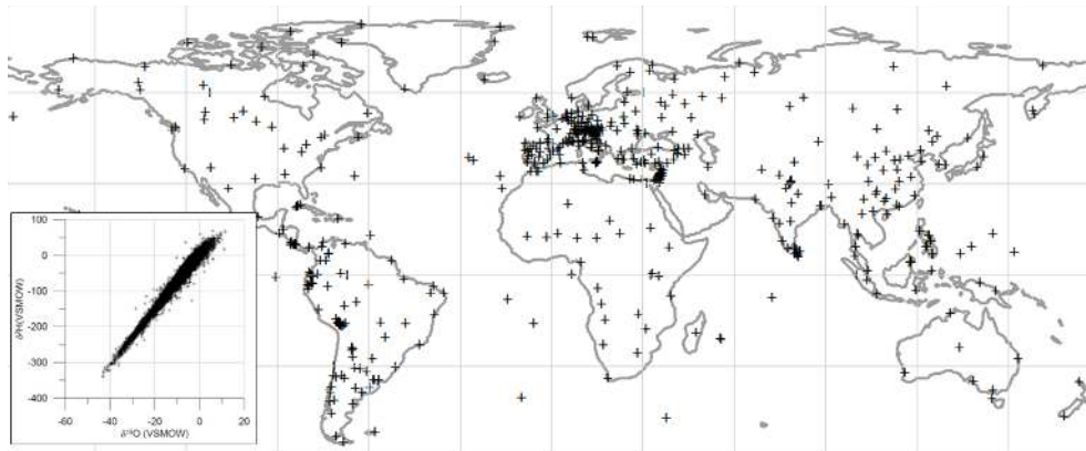
Fig. 1. Global map of GNIP stations used for RCWIP modeling. All stations represented 2 to 52 yr of monthly \delta^{18}\text{O} or \delta^2\text{H} and climate data from 1960 to 2009. Inset: a cross-plot of \delta^{18}\text{O} versus \delta^2\text{H} at stations used, yielding a GMWL of \delta^2\text{H} = 7.91 \delta^{18}\text{O} + 8.72 ( R^2 = 0.976 , n = 576 ).
