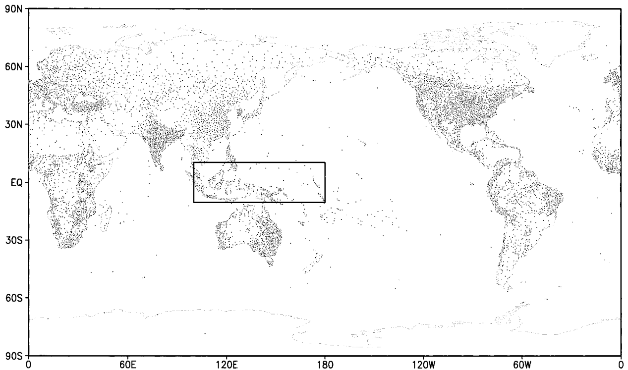
FIG. 2. Distribution of the gauge stations with 10-yr-or-longer recording periods from 1951 to 1990 collected in the GHCN2 and CAMS datasets. The labeled box indicates the subregion of the Indonesian islands (see text).
