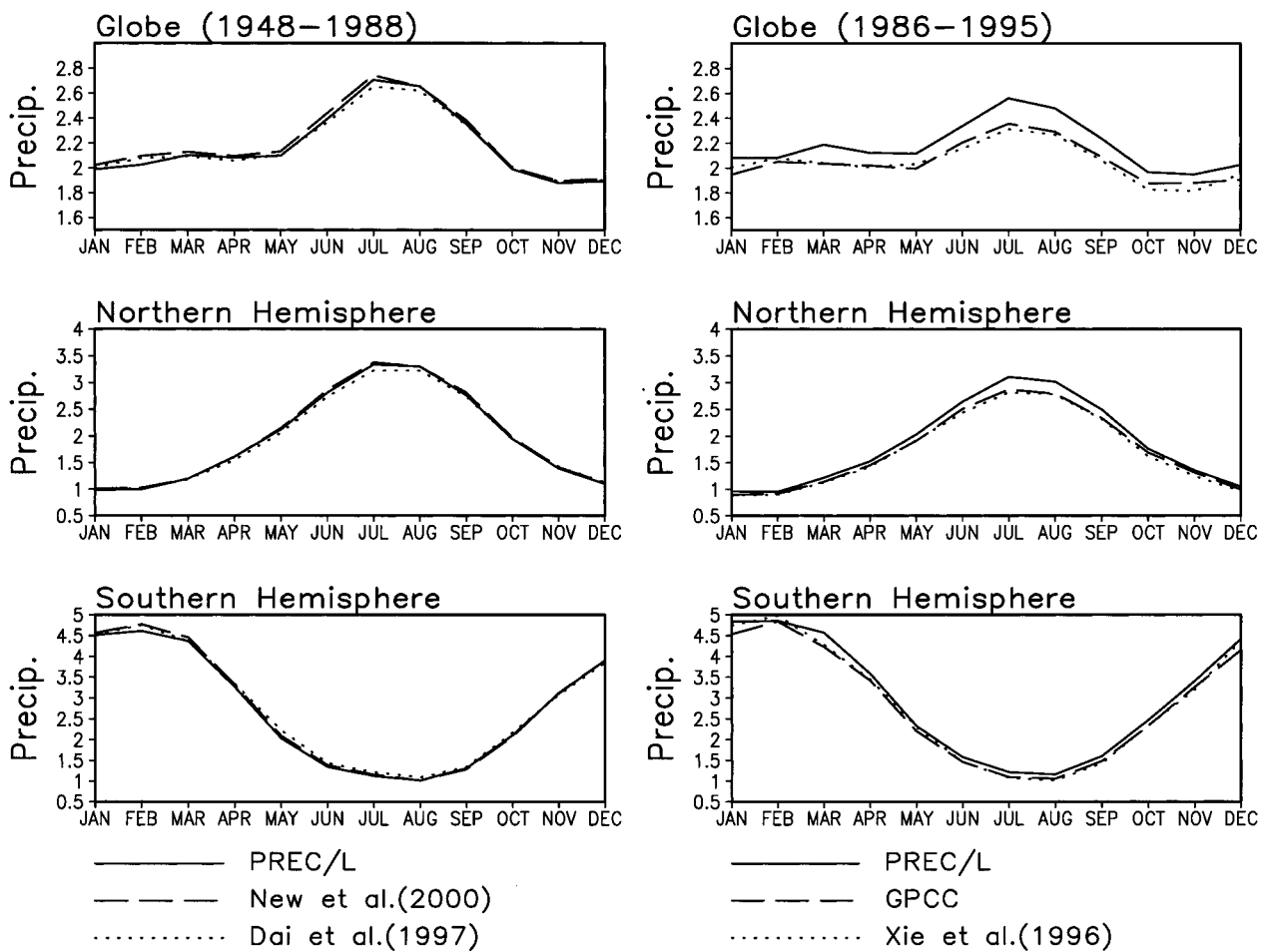
FIG. 7. Annual cycles of mean precipitation (mm day -1 ) over 2.5° latitude/longitude grid boxes with at least 50% land coverage over (top) the entire globe, and the (middle) Northern and (bottom) Southern Hemispheres as defined by several datasets. (left) The results for the 41-yr period from 1948 to 1988. (right) Those for the 10-yr period from 1986 to 1995.
