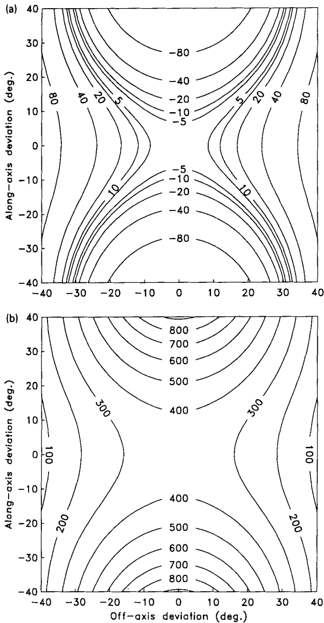
Figure 24. (a) The change in traveltime resulting from perturbations in the SS bounce-point position at a source-receiver range of 140^\circ . The Fresnel zone for 20 s waves is given by the \pm 5 s contours. (b) Apparent discontinuity depth as a function of distance away from a single point scatterer at 350 km.
