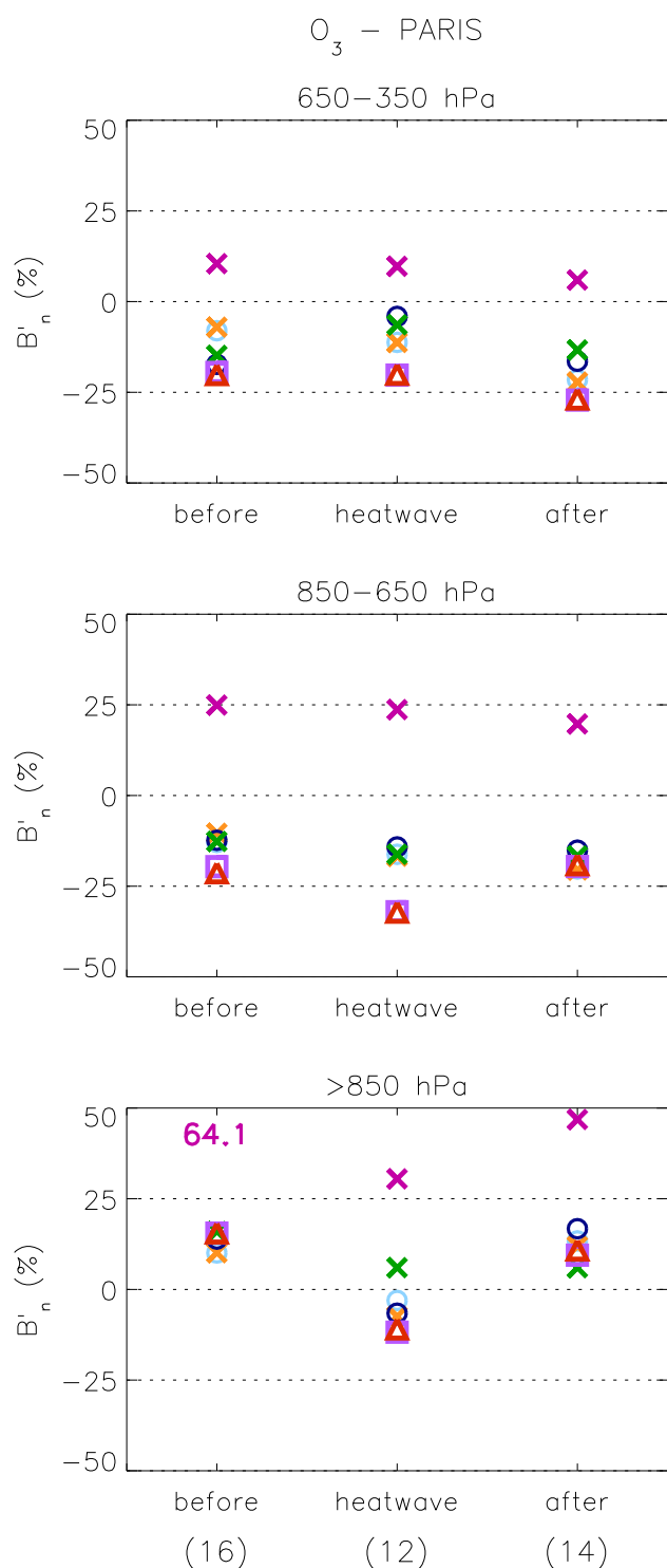
Fig. 7. As Fig. 6 but only for O_3 above Paris. In the case of MOZART for the lowest layer before the heat wave, the numerical value of B'_n is explicitly indicated because it is outside the plotting area.
