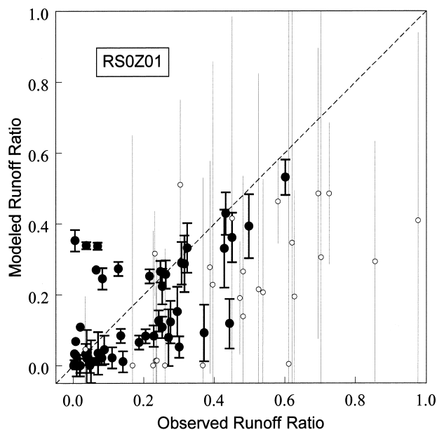
FIG. 9. Scatterplot of modeled runoff ratio against observed runoff ratio for the RS0Z01 experiment (i.e., like NEW, but with r_s = 0 and z_o = z_T = 0.01 m). Error bars denote \pm 1 characteristic error ( \Delta^* ) in runoff ratio resulting from error of precipitation. For clarity, basins with \Delta^* smaller than 0.1 are plotted with filled symbols and heavy error bars.
