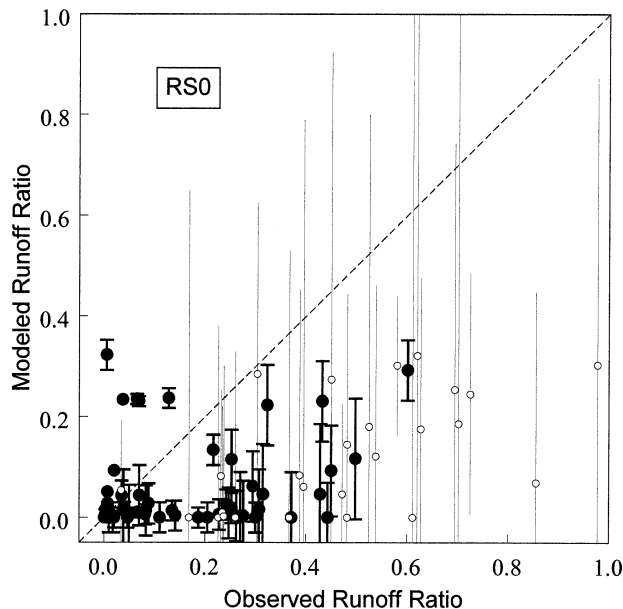
FIG. 8. Scatterplot of modeled runoff ratio against observed runoff ratio for the RS0 experiment (i.e., like NEW, but with r_s = 0 ). Error bars denote \pm 1 characteristic error ( \Delta^* ) in runoff ratio resulting from error of precipitation. For clarity, basins with \Delta^* smaller than 0.1 are plotted with filled symbols and heavy error bars.
