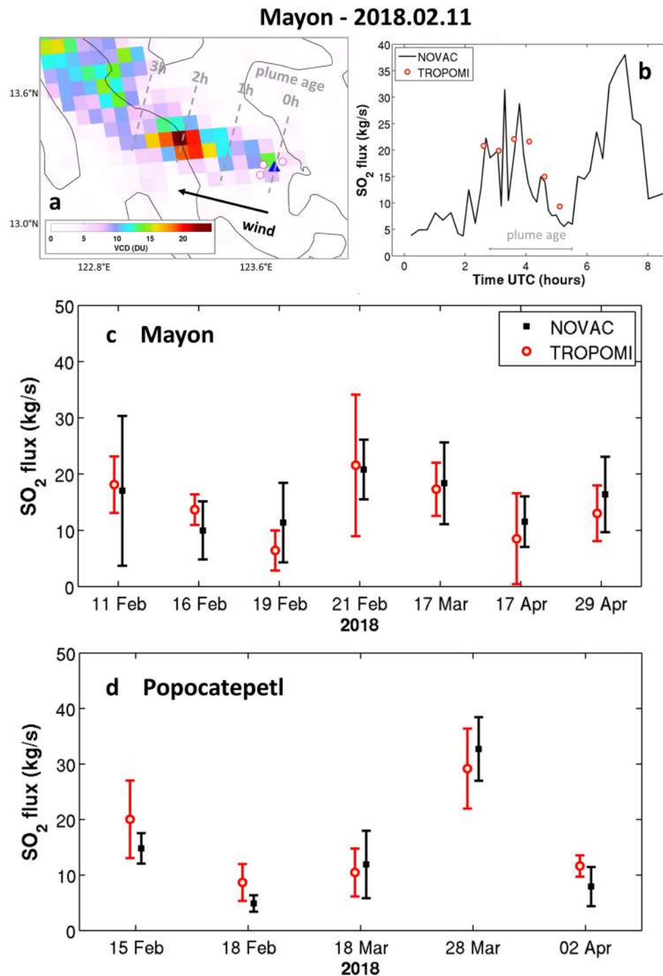
Figure 5. Panels a and b illustrate the TROPOMI \text{SO}_2 flux retrieval technique for the case of Mayon (13.26°N, 123.68°E) on February 11, 2018. (Panel a) TROPOMI \text{SO}_2 VCDs (DU) over the island of Luzon (Philippines), the Mayon volcano is symbolized by a blue triangle, the locations of the NOVAC instruments are marked by magenta circles. From the plume direction and wind speed at plume altitude, a plume age (expressed in hour) is assigned to each TROPOMI pixel. (Panel b) TROPOMI \text{SO}_2 flux (kg/s) obtained at half-hourly sampling from the traverses downwind (hence back in time as illustrated by the gray arrow representing the plume age) and comparison with NOVAC \text{SO}_2 time-series. (Panels c,d) \text{SO}_2 fluxes retrieved from selected days of TROPOMI data for February–April 2018 period, for Mayon and Popocatepetl (19.02°N, 98.63°W) respectively, and estimations from NOVAC measurements. Mean \text{SO}_2 fluxes and standard deviation are depicted for each day.
