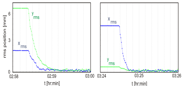
Figure 3: Measured orbit rms in both accelerators in the horizontal (x) and vertical (y) planes.
