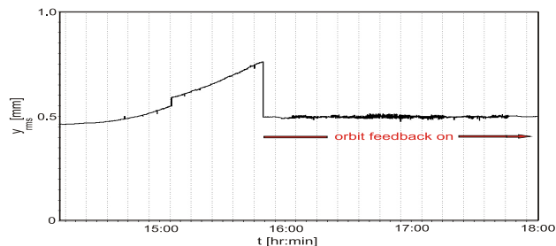
Figure 6: Measured vertical orbit rms versus time without feedback evidencing drift, then with feedback engaged.
