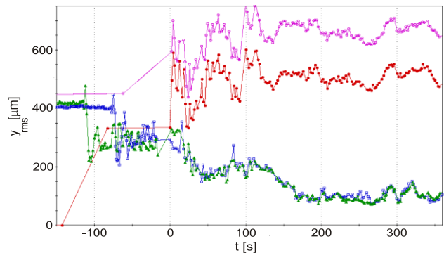
Figure 4: Vertical orbit rms during energy ramp measured with (blue, green) and without (red, pink) global orbit feedback versus time.
