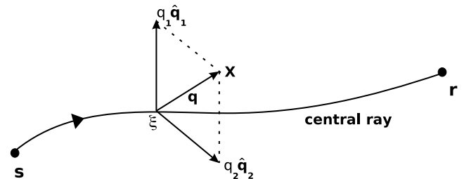
Figure 3. Perpendicular projection of a scatterer x onto the paraxial point \xi , situated on the central geometrical ray from the source s to the receiver r . The off-path difference vector is expressed in terms of two orthogonal unit vectors: q = q_1 \hat{q}_1 + q_2 \hat{q}_2 . The ray-centred coordinates of the scatterer are x = (q_1, q_2, l) where l is the arc length along the central ray (Dahlen et al. 2000).
