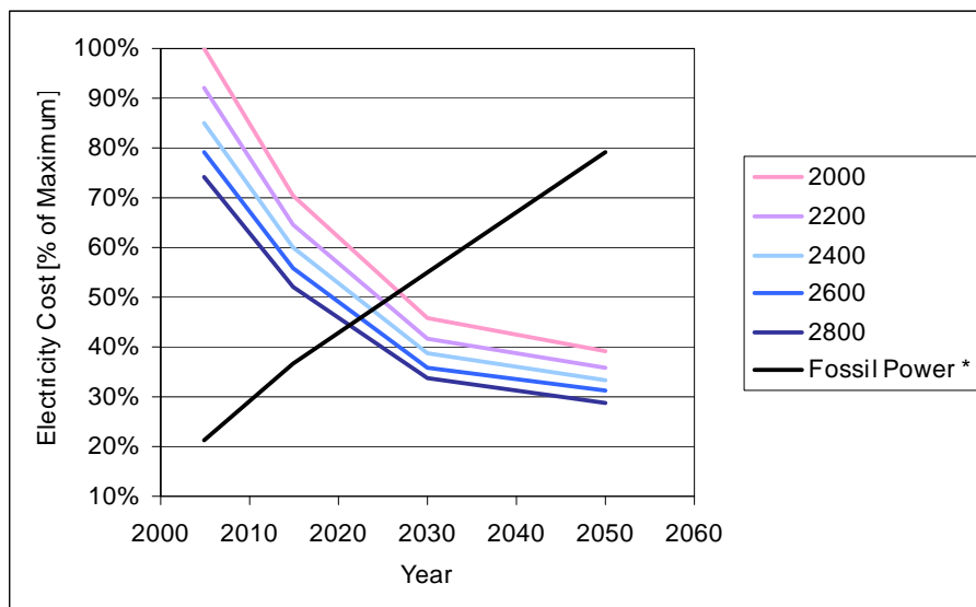
Fig. 8. Electricity cost in % of the maximum starting value in 2005 as function of time and direct normal irradiation (DNI in kWh/m 2 /y) for CSP reference plants with a solar multiple SM4 compared to the cost of power generation from fossil fuels (including carbon costs) according to [9]*
