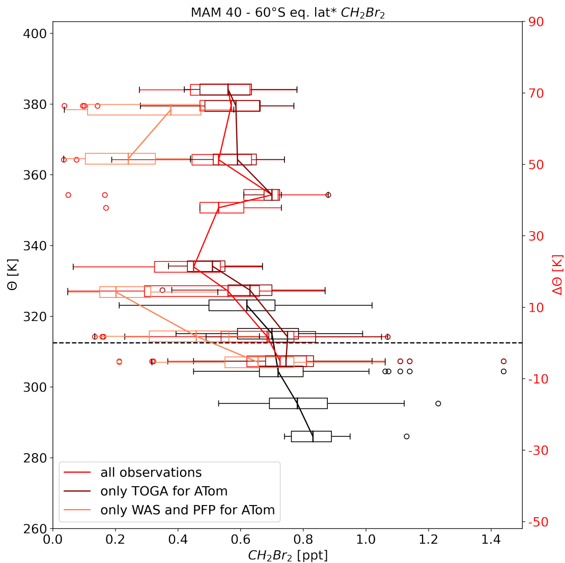
Figure 8. As in Fig. 7, but only \text{CH}_2\text{Br}_2 for SH autumn. Profile as a function of potential temperature difference to the local tropopause was split into three profiles. Profile using all observations is in red, similar to Fig. 7, profile using all observation but with only TOGA observations from ATOm in dark red and profile using all observations but with only flask observations in light red.
