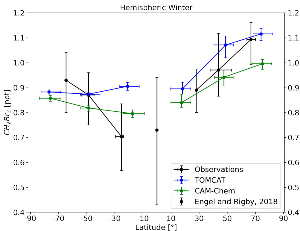
Figure 5. Latitude cross section of tropopause representative mixing ratios of \text{CH}_2\text{Br}_2 from observation and model results for both hemispheres in winter. Data are binned into three latitude bins for each hemisphere: high latitudes (60-90°), mid latitudes (30-60°), and low latitudes (0-30°) and only for data within the 10 K below the dynamical tropopause. Shown are the medians with the error bars representing the interquartile range (IQR). The median latitudinal position of observational and model bins may differ due to different spatial data coverage of observations and models. Also included is the reference mixing ratio for the tropical tropopause (Engel and Rigby, 2018).
