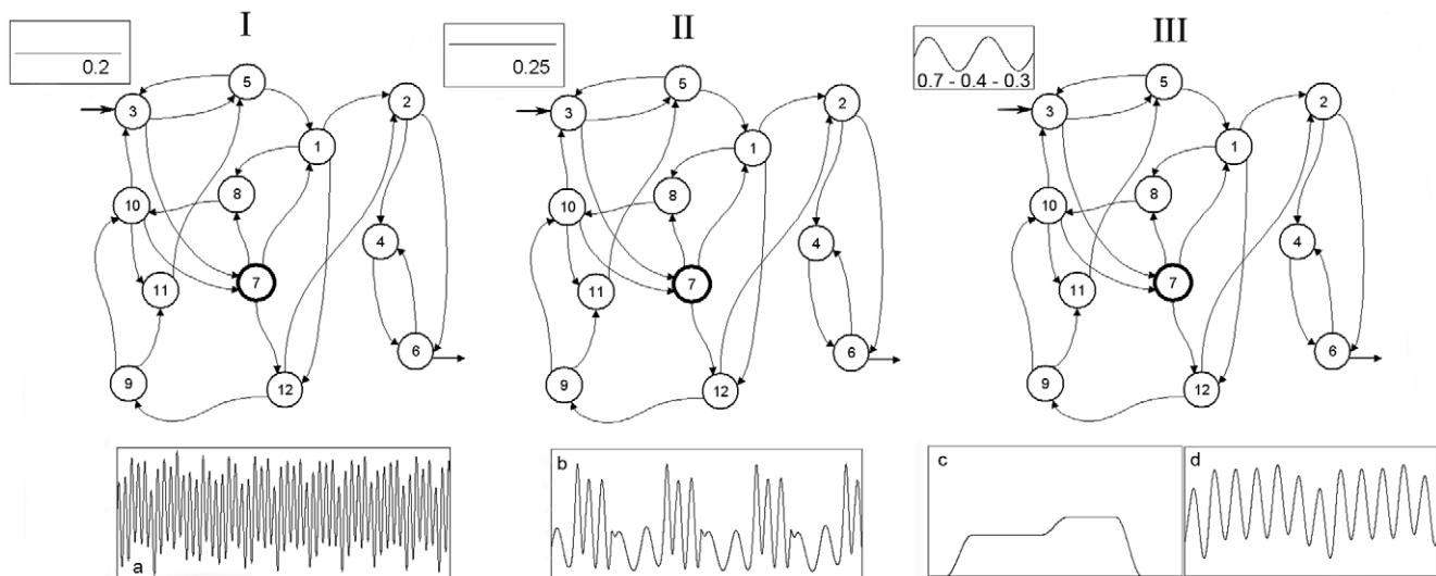
Figure 2. Summary of the numerical experiments. The DMN was perturbed by three different values of the external input flux belonging to the metabolic subsystem number three. I: Chaotic patterns emerge under a stationary external input flux of substrate with a baseline of 0.2 (figure 2a). II: Under a stationary input flux with a baseline of 0.25, the network undergoes a reorganization of its dynamics and spontaneously all the subsystems present complex regular behaviours in their activities (figure 2b). III: Finally, we have considered an oscillatory external input flux (baseline: 0.7, amplitude: 0.4 and frequency: 0.3) and in the metabolic subsystems steady-state patterns (figure 3c) and simple regular transitions between different periodic oscillations (figure 3d) emerge. Circles with thin line represent subsystems always locked into active states, while the circle with thick line represents a metabolic subsystem with dynamics on-off. doi:10.1371/journal.pone.0009484.g002
