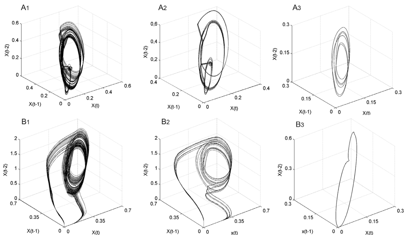
Figure 4. Local attractors in the dissipative metabolic network. The dynamical reorganizations of the network are represented by local attractors which are the set of possible asymptotic behaviours for each metabolic subsystem activity. The first row (A1, A2 and A3) corresponds to subsystem number two during the changes provoked by three different patterns in the external input fluxes, and the second row (B1, B2 and B3) corresponds to subsystem number seven.
