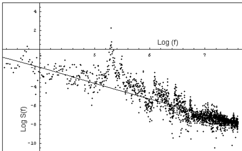
Figure 5. Spectral density plot of a representative series of the dissipative metabolic network. S(f) is the absolute value of the Fourier transform and f the frequency. The opposite of the slope has a value of 1.663; this means that the process is a fractional Brownian motion (fBm). doi:10.1371/journal.pone.0009484.g005
