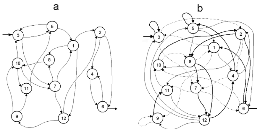
Figure 1. Topology of the metabolic network. Dissipative metabolic network formed by 12 subsystems in which the interconnection by substrate fluxes (figure 1a) and input regulatory signals (figure 1b) are reflected. These regulatory signals, allosteric activation (thin line), allosteric inhibition (thick line) and covalent modulation of total inhibition (dashed line), come from any element of the network and do not require any flux relationship.
