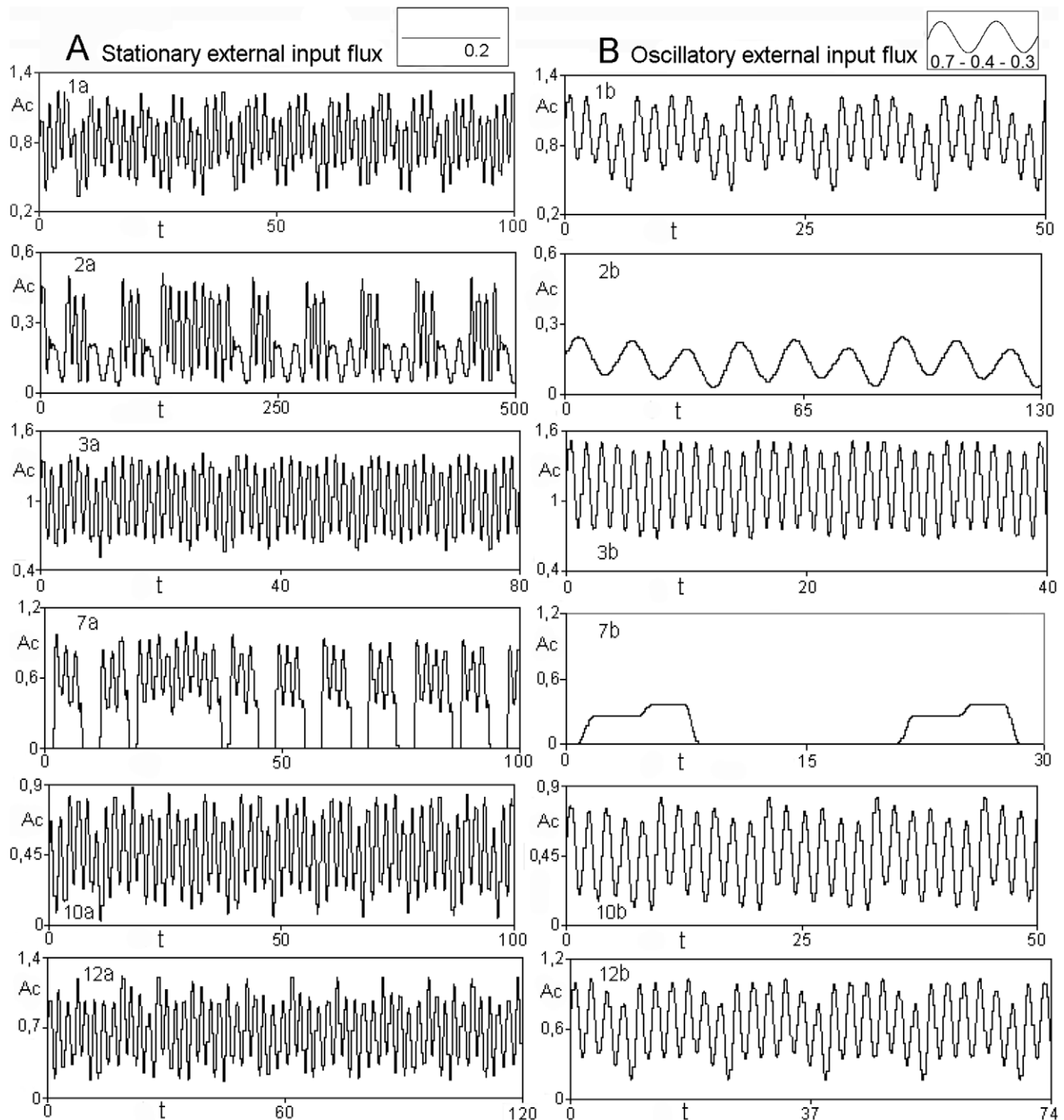
Figure 3. Emergent dynamic behaviours in the dissipative metabolic network. A: chaotic series, the metabolic subsystems show infinite transitions between different activity patterns when the network is perturbed by a stationary external input flux of substrate (baseline of 0.2). B: regular transitions between periodic or steady state behaviours emerge when the network is perturbed by an oscillatory external input flux of substrate (baseline: 0.7, amplitude: 0.4 and frequency: 0.3). The activity A_c developed by each metabolic subsystem is represented as a function of the time t . doi:10.1371/journal.pone.0009484.g003
