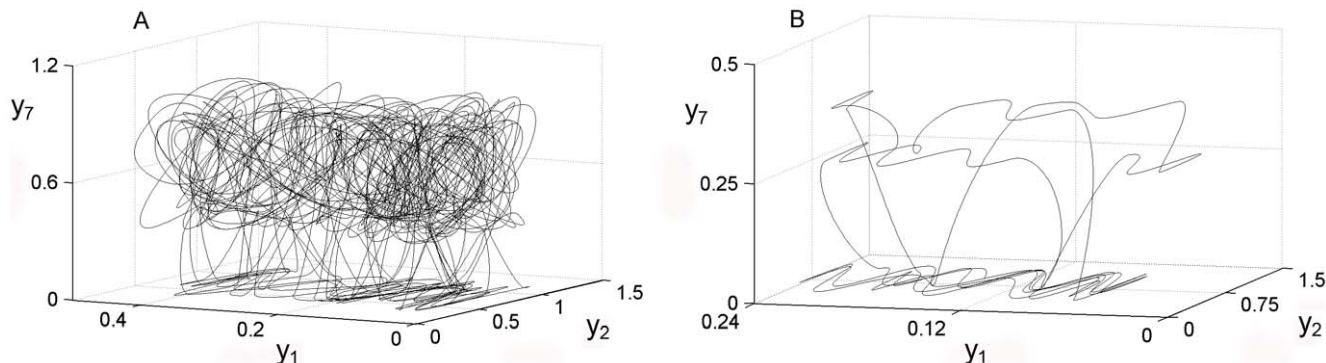
Figure 6. Global attractors in the dissipative metabolic network. 4A: chaotic global attractor which emerge when the network is perturbed by a stationary external input flux of substrate with a baseline of about 0.2. Figure 4B shows a regular global attractor, i.e. the set of biochemical states when the network is perturbed by an oscillatory external input of substrate. We have represented their projections in only three dimensions for the metabolic subsystems 1, 3 and 4 (the x-axis is the 1a series, the y-axis is the 3a series, and the z-axis is the 4a series).
