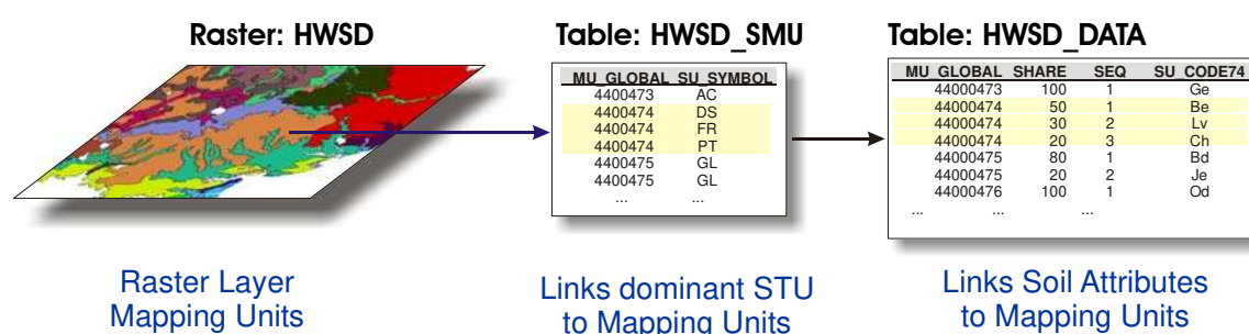
Figure 1: Schematic Organization of Spatial and Typological Units in Harmonized World Soil Database
