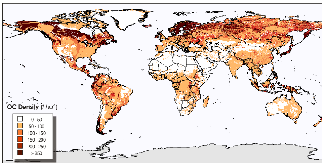
Figure 16: Soil Organic Carbon Density ( t\ ha^{-1} ) for Combined Topsoil and Subsoil Layer (0 – 100cm) from HWSD V1.1
