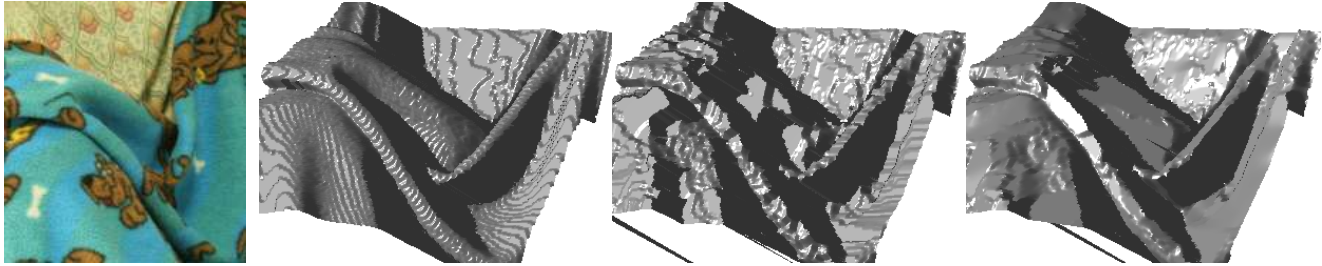
Figure 8. Curved surfaces. Left to right: T_0 for the Middlebury “Cloth3” sequence, ground truth (discretized) disparity surface (3-d view of disparity map), disparity surfaces generated using Smooth* proposals and 1op and 2op respectively. (Spurious pixels have been fixed to the back-plane, for improved visualization.)
