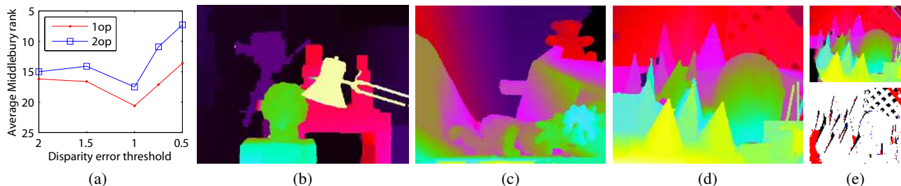
Figure 7. Middlebury performance. (a) A graph of average rank on the Middlebury stereo evaluation, against disparity error threshold, for both first and second order priors. (b)–(d) Output disparity using “2op, Smooth”, QPBOI-R, \delta E_{\text{thresh}} = 0.01\% ”, for the Middlebury “Tsukuba”, “Teddy” and “Cones” sequences respectively. (e) Top : Output disparity using the same method as (d), but with no visibility constraint ( i.e. V_i(\mathbf{x}) = 1 \forall \mathbf{x} ). Bottom : Visibility map for \mathcal{I}_1 of “Cones”—pixels deemed occluded according to the following disparity maps are painted (covering the previous color) in the following order: disparity map above, red; (d), blue; ground truth, black.
