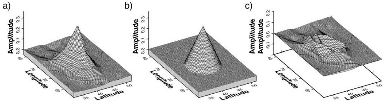
Figure 13. Resolution method. (a) For each grid point on the globe we construct the resolution kernel, which is a row of the resolution matrix and can be presented as a map. (b) We fit a cone to the kernel and identify the resolution with the full width at half maximum height of the cone. (c) Typically, a cone fits well, as shown by the difference between the resolution kernel and best fitting cone. For perfect resolution, the resolution kernel would have a single nonzero point, implying a resolution of M \times 111 km on a M^\circ \times M^\circ grid.
