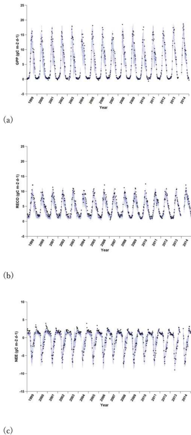
Fig. 7 Fitting of GPP (a), RECO (b), and NEE (c) of site DK-SOR (55.4859°N, 11.6446°E). Dark dots represent measurements, horizontal blue bars represent the means (predictions) and vertical blue lines are the standard deviations of flux values in the terminal nodes of 500 trees.
