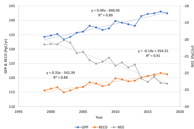
Fig. 5 Trend of global annual GPP, RECO, and NEE (PgC yr -1 ). An annual mean is the global integral of fluxes in 0.1° × 0.1° grids.
