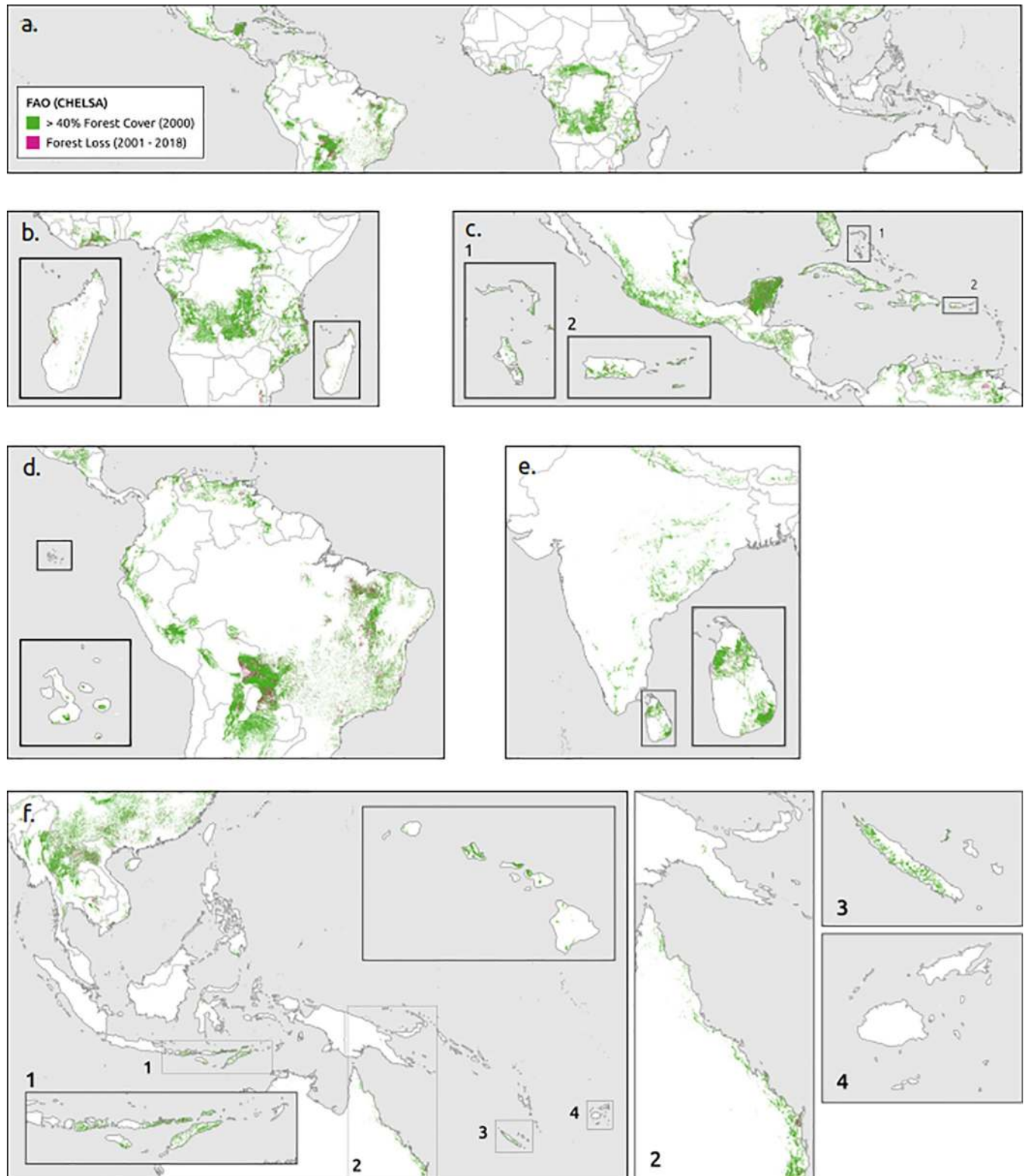
Fig 5. Forest cover and change from FAO bioclimatic definition, CHLSA climate data set, and closed canopy cover. (a) Global, (b) Africa, (c) North and Central America, (d) South America, (e) South Asia, and (f) Southeast Asia & Asia Pacific.
