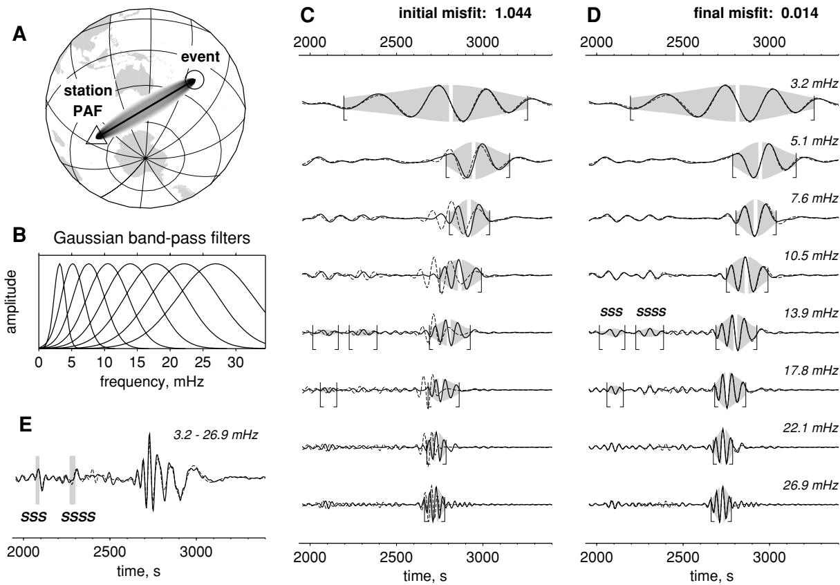
Figure 2. Automated multimode inversion. (a) An earthquake on 1996 August 5 ( 15^{\circ}\text{S} , 173^{\circ}\text{W} , 54 km depth, M_w = 6.6 ) was recorded on the vertical component at the station PAF (Port aux Français, Kerguelen Island) operated by Geoscope; the source-station distance is 10 569 km. The plots are as in Fig. 1 except with eight Gaussian filters, 11 time-frequency windows, and arrivals of the SSS and triplicated SSSS waves labelled.
