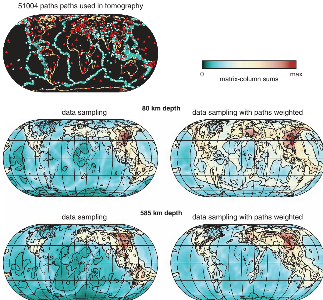
Figure 8. Top: the dense coverage of the globe with the \sim 51\,000 source-station paths. Earthquakes used are plotted as circles, stations as triangles. Below: relative data sampling without and with path weighting at two depths. The measure of data sampling is the sums of the columns of the matrix that relates the data to the model, with each column corresponding to one parameter. We plot sums of shear-velocity-parameter columns. The colour-scale limits are different for every frame, scaled to the maximum of each distribution.
