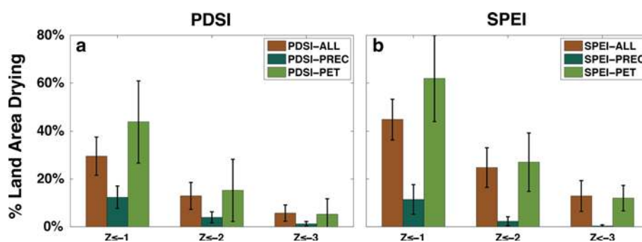
Fig. 13 Percent land area (excluding Antarctica) with annual average 2080–2099 PDSI (a) and SPEI (b) exceeding 1, 2, or 3 standard deviations. Bars represent the multi-model mean, and the error bars
