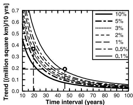
Fig. 3. Estimated probabilities of observed or larger trend occurrence in NH sea ice extent for specified time intervals. Estimates are based on the GFDL climate model's 5000-year control run. Circle corresponds to the observed 46-year (1953–98) trend of -0.19 \times 10^6 \text{ km}^2 per 10 years (13). The probability for such a trend to occur by chance as the result of natural climate variability is <0.1\% . Square corresponds to the observed 19.4-year (1978–98) trend of -0.37 \times 10^6 \text{ km}^2 per 10 years (16). The probability of such a trend occurring by chance as the result of natural climate variability is <2\% .
