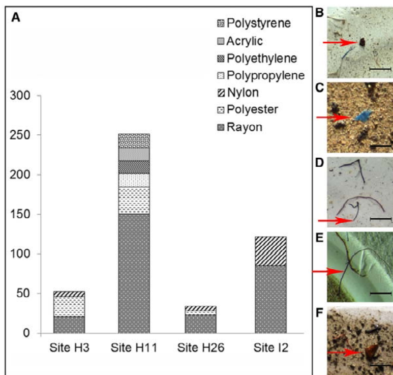
Figure 2. (A) Total number of microplastic pieces presented as values per cubic meter of seawater (scaled up from sample volumes examined which were typically 50-100 cm 3 ), by polymer type, according to the location of sea ice cores. Photographs of microplastic fragments, identified using FT-IR: (B) HOTRAX Site 3, polyethylene terephthalate (polyester), (C) HOTRAX Site 11, polypropylene, (D) HOTRAX Site 26, polyester, (E) ICESCAPE Site 2, nylon, (F) HOTRAX Site 11, polyethylene. Scale bars represent 1 mm.
