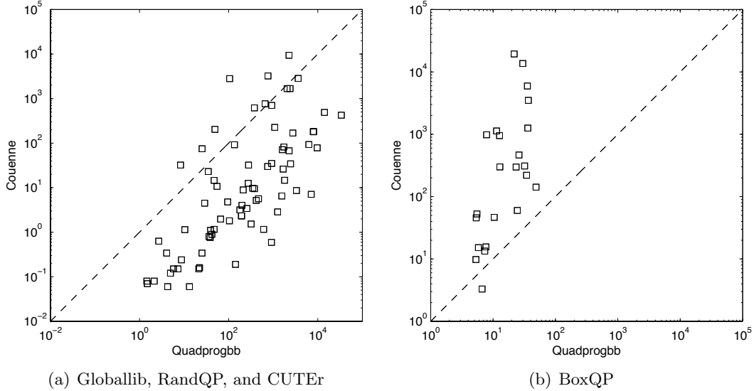
Figure 2: CPU times – QUADPROGGB vs. Couenne
