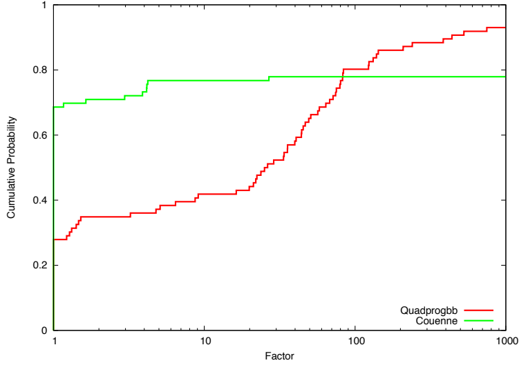
(a) Globallib, RandQP, and CUTer
