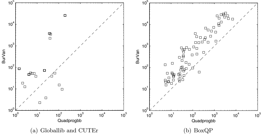
Figure 1: CPU times – QUADPROGGB vs. BURVAN
