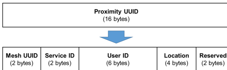
Figure 5. User’s presence state from the Mobile App is embedded in the Proximity universally unique identifier (UUID) field of a standard iBeacon message.
