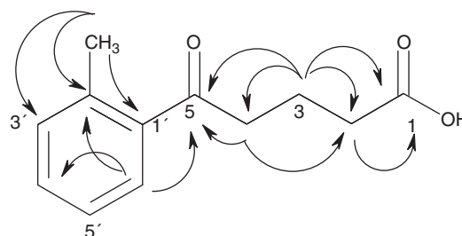
Figure 2 (→) HMBC connectivities of 5-oxo-5- o -tolyl-pentanoic acid ( 8a ).
