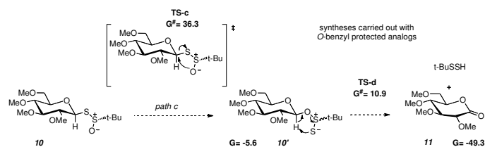
Figure 2. 1,3 Shift of the thiosulfinate group in 10 , followed by E i elimination ( path c ). \Delta G in kcal.mol -1
