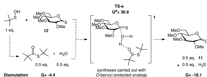
Figure 3. Dismutation of tert -butyl sulfenic acid, followed by hydrolysis of thionolactone 12 . \Delta G in kcal.mol -1
