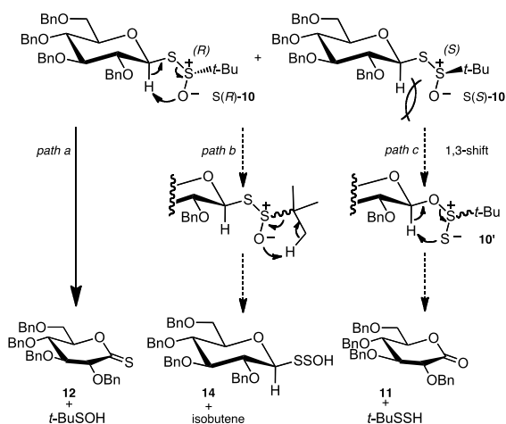
Scheme 3: Possible reaction paths for the thermolysis of D-glucosyl tert -butyl thiosulfates 10
