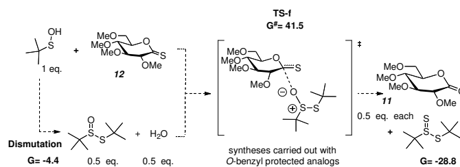
Figure 4. Dismutation of tert -butyl sulfenic acid, and di- tert -butyl thiosulfinate attacking thionolactone 12 . \Delta G in kcal.mol -1
