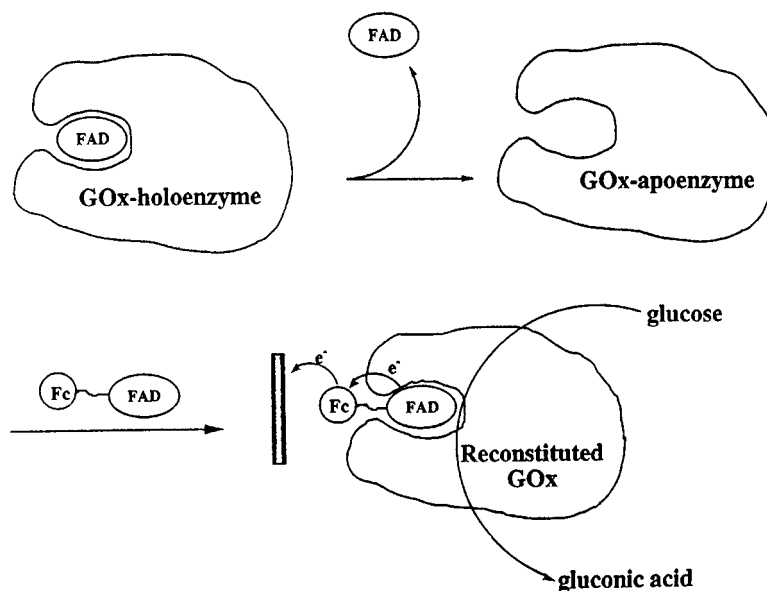
Fig. 3. Electrical contacting of a flavoenzyme by its reconstitution with a relay-FAD semisynthetic cofactor. (Reproduced with permission [29b]).
