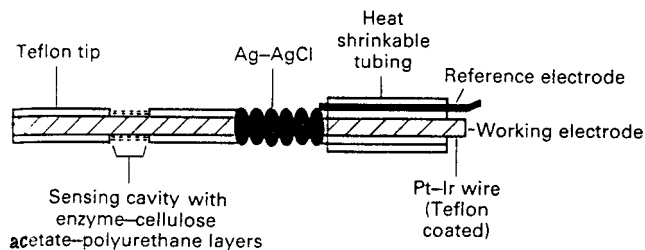
Fig. 4. A needle-type glucose biosensor for subcutaneous monitoring (reproduced with permission [14]).
