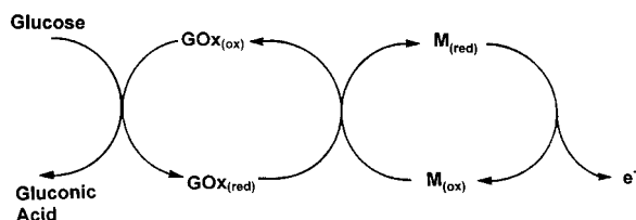
Fig. 2. Sequence of events that occur in 'second-generation' (mediator-based) glucose biosensors mediated system.
