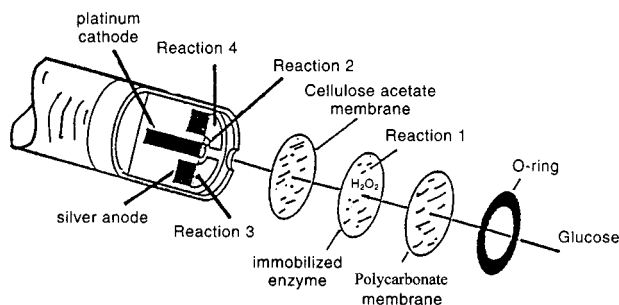
Fig. 1. Schematic of a “first-generation” glucose biosensor (based on a probe manufactured by YSI Inc.).
