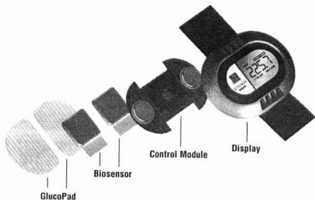
Fig. 5. Various components of the watch-like glucose monitor being developed by Cygnus Inc.
