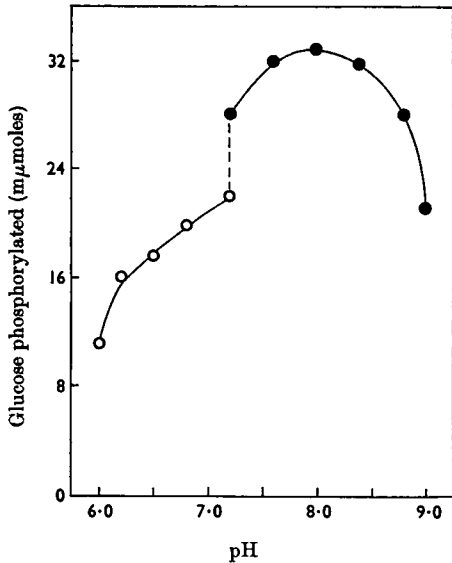
Fig. 1. Variation of hexokinase activity with pH value of incubation medium. ○, Tris phosphate buffer; ●, tris-HCl buffer.
