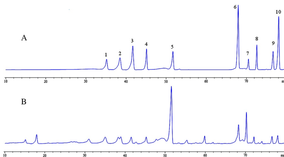
Figure 2 HPLC chromatogram of flavonoid compositions in flavonoid compound (FC). (A) standard flavonoids; (B) FC. Peaks: 1: vitexin; 2: rutin; 3: hyperoside; 4: luteolin-7-O- \beta -D-glucopyranoside; 5: quercitrin; 6: quercetin; 7: tiliroside; 8: luteolin; 9: apigenin; 10: kaempferol.
