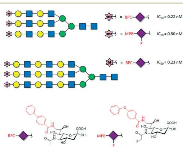
Fig. 6 Trivalent modified N -glycans described as pM inhibitors of Siglec-2.
