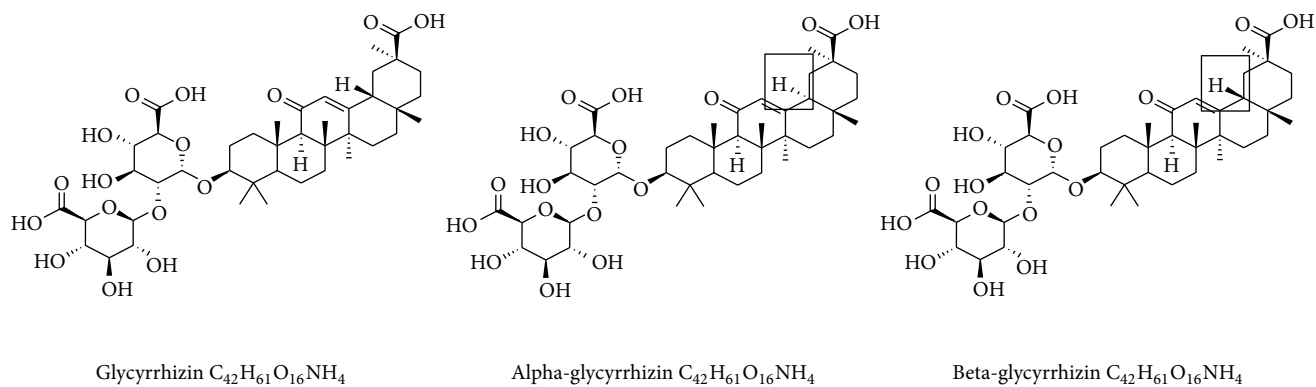
FIGURE 1: Chemical structure of glycyrrhizin (GA) and its derivatives.
