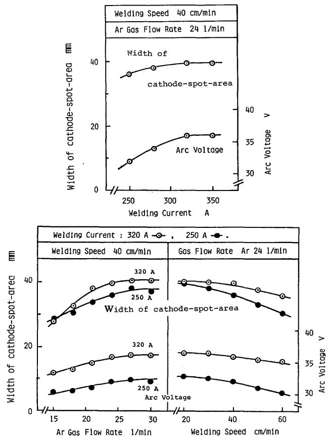
Fig. 4 Changes in width of cathode-spot-area under various conditions of welding current, argon gas flow rate and welding speed.
