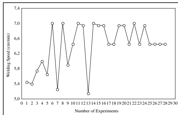
Figure 5. Convergence of the welding speed.
