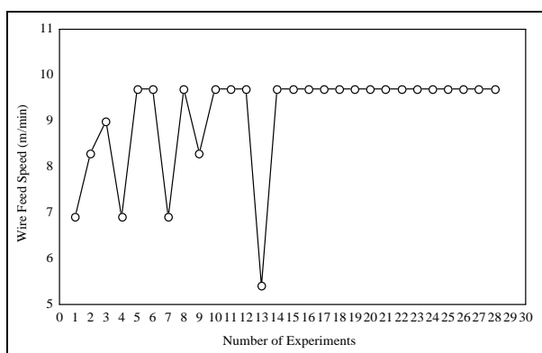
Figure 4. Convergence of the wire feed speed.
