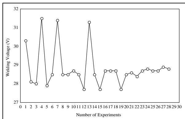
Figure 3. Convergence of the welding voltage.
