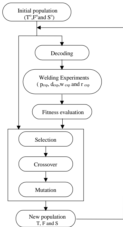
Figure 1. The GMAW welding optimization procedure using genetic algorithm.
