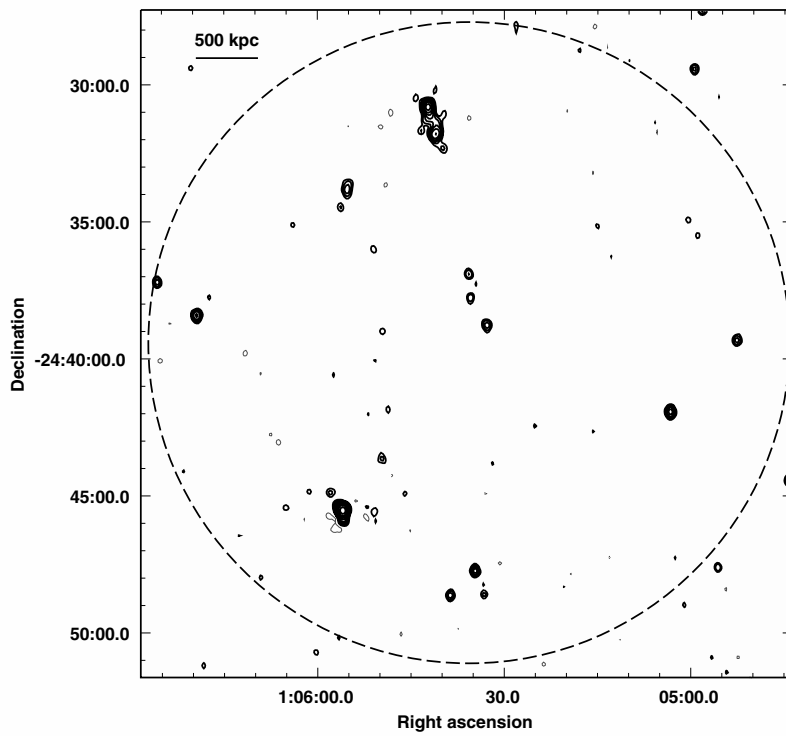
Fig. A.7. GMRT 610 MHz radio contours for the cluster A 141. The 1\sigma level in the image is 90 \mu\text{Jy b}^{-1} . Contours are 0.45 \times (\pm 1, 2, 4, 8, 16\dots) \text{mJy b}^{-1} . The HPWB is 15'' \times 12'' , PA 0^\circ . The radius of the dashed circle is the virial radius, corresponding to 11.79' for this cluster.
