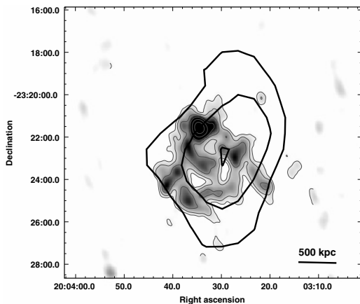
Fig. 7. ROSAT All Sky Survey contours (black) of RXCJ 2003.5–2323 overlaid on the 610 MHz gray scale and contours (gray) of the radio halo. The X-ray contours levels are logarithmically spaced by a factor of \sqrt{2} . The radio image is the same as right panel of Fig. 6.
