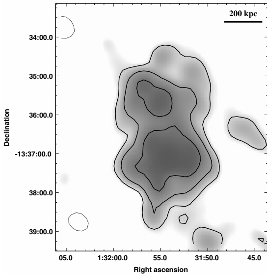
Fig. 3. Radio contours over grey scale of the A209 cluster radio halo after subtraction of the individual radio sources (see left panel of Fig. 2 and Sect. 4.1.1 in the text). The resolution of this image is 32.0'' \times 30.0'' , PA 30^\circ . The rms ( 1\sigma ) in the image is 0.15 \text{ mJy b}^{-1} , contours are 0.35 \times (\pm 1, 2, 4, 8, 16\dots) \text{mJy b}^{-1} .
