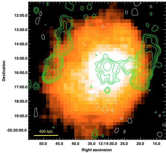
Fig. 5. GMRT 610 MHz radio contours for the cluster RXCJ 1314.4–2515 superposed on the X-ray archive ASCA image (colour). The 1\sigma level in the image is 60 \mu\text{Jy b}^{-1} . Contours are 0.18 \times (\pm 1, 2, 4, 8, 16\dots) mJy \text{b}^{-1} . The HPWB is 25.0'' \times 22.0'' , PA 15^\circ .
