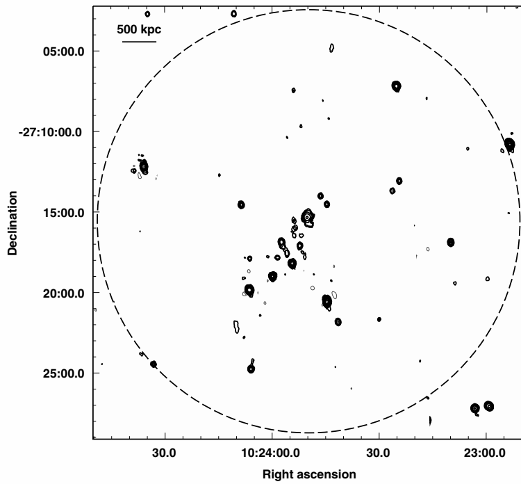
Fig. A.4. GMRT 610 MHz radio contours for the cluster A 3444. The 1\sigma level in the image is 60 \mu\text{Jy b}^{-1} . Contours are 0.4 \times (\pm 1, 2, 4, 8, 16\dots) \text{mJy b}^{-1} . The HPWB is 15'' \times 12'' , PA 0^\circ . The radius of the dashed circle is the virial radius, corresponding to 13.14' for this cluster.
