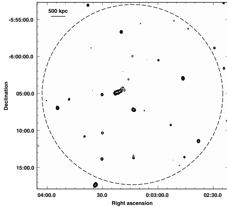
Fig. A.6. GMRT 610 MHz radio contours for the cluster A 2697. The 1\sigma level in the image is 80 \mu\text{Jy b}^{-1} . Contours are 0.4 \times (\pm 1, 2, 4, 8, 16\dots) \text{mJy b}^{-1} . The HPWB is 15'' \times 12'' , PA 0^\circ . The radius of the dashed circle is the virial radius, corresponding to 12.17' for this cluster.
