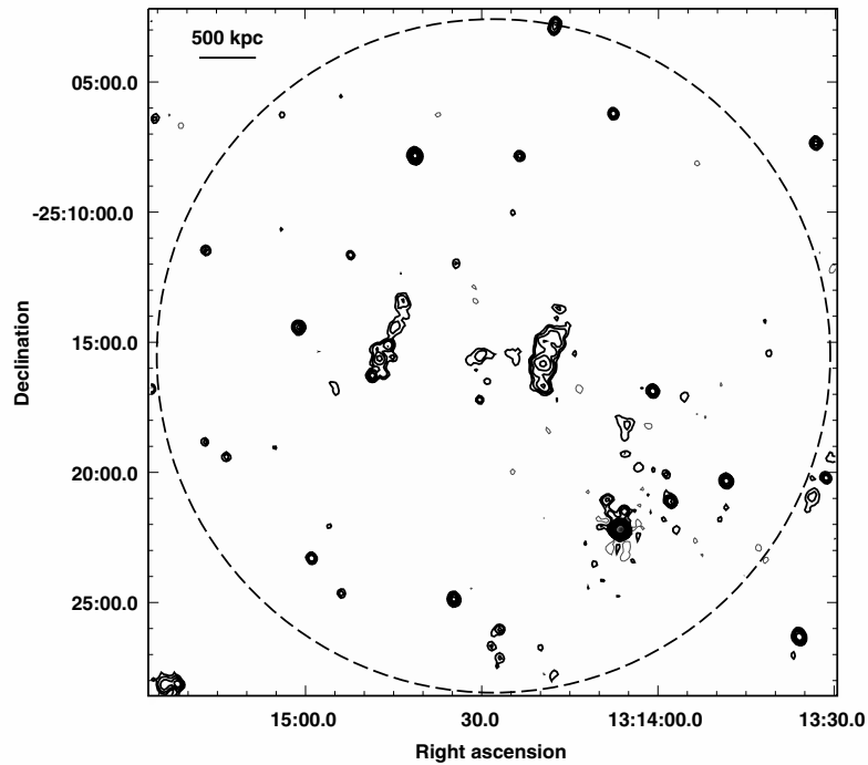
Fig. A.2. GMRT 610 MHz radio contours for the cluster RXCJ 1314.4–2515. The 1\sigma level in the image is 60 \mu\text{Jy b}^{-1} . Contours are 0.3 \times (\pm 1, 2, 4, 8, 16\dots) \text{mJy b}^{-1} . The HPWB is 15.0'' \times 13.0'' , PA 15^\circ . The radius of the dashed circle is the virial radius, corresponding to 12.94' for this cluster.
