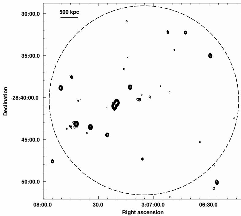
Fig. A.8. GMRT 610 MHz radio contours for the cluster A 3088. The 1\sigma level in the image is 65 \mu\text{Jy b}^{-1} . Contours are 0.325 \times (\pm 1, 2, 4, 8, 16\dots) \text{mJy b}^{-1} . The HPWB is 15'' \times 12'' , PA 0^\circ . The radius of the dashed circle is the virial radius, corresponding to 11.36' for this cluster.
