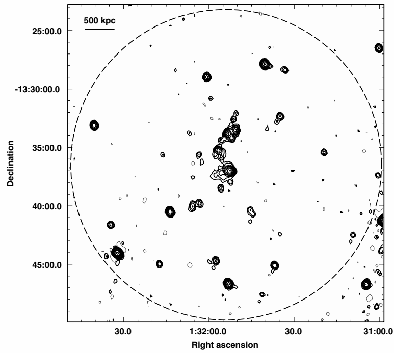
Fig. A.1. GMRT 610 MHz radio contours for the cluster A209. The 1\sigma level in the image is 50 \mu\text{Jy b}^{-1} . Contours are 0.20 \times (\pm 1, 2, 4, 8, 16\dots) \text{mJy b}^{-1} . The HPWB is 21.0'' \times 18.0'' , PA 13^\circ . The radius of the dashed circle is the virial radius, corresponding to 13.28' for this cluster.
