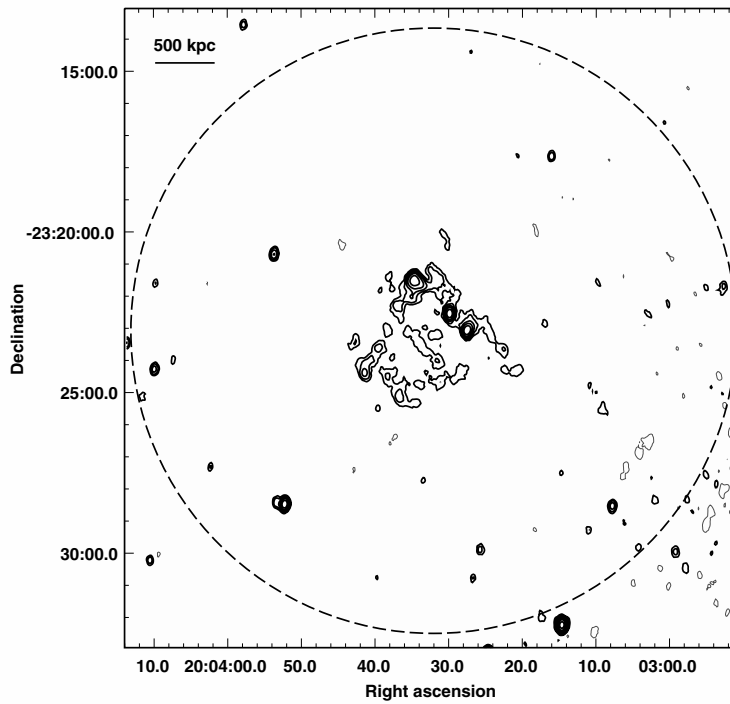
Fig. A.3. GMRT 610 MHz radio contours for the cluster RXCJ 2003.5-2323. The 1\sigma level in the image is 60 \mu\text{Jy b}^{-1} . Contours are 0.3 \times (\pm 1, 2, 4, 8, 16\dots) \text{mJy b}^{-1} . The HPWB is 15.5'' \times 10.3'' , PA -6^\circ . The radius of the dashed circle is the virial radius, corresponding to 9.91' for this cluster.
