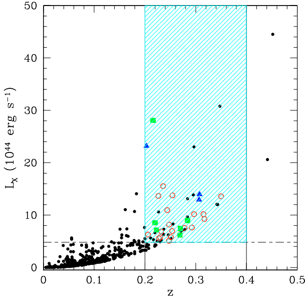
Fig. 1. L_x - z plot (0.1–2.4 keV) for the REFLEX clusters. Open red circles show the clusters selected for the GMRT observations of the present project (marked with the symbol \surd in Table 1; see Sect. 3 for details); filled blue triangles indicate those clusters (marked with * in Table 1) which are known to host a radio halo from the literature, i.e. A 2744 (Govoni et al. 2001), A 1300 (Reid et al. 1999) and A 2163 (Herbig & Birkinshaw 1994; Feretti et al. 2001); filled green squares indicate the clusters of the sample belonging to the GMRT Cluster Key Project (P.I. Kulkarni). The light blue dashed region is the one surveyed in our project.
