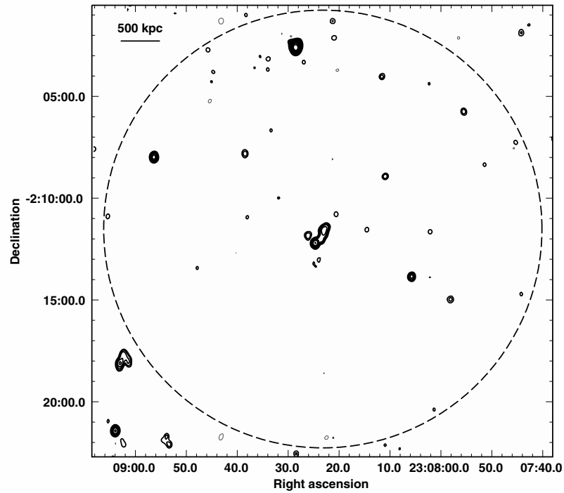
Fig. A.9. GMRT 610 MHz radio contours for the cluster A2537. The 1\sigma level in the image is 80 \mu\text{Jy b}^{-1} . Contours are 0.4 \times (\pm 1, 2, 4, 8, 16\dots) \text{ mJy b}^{-1} . The HPWB is 15'' \times 12'' , PA 0^\circ . The radius of the dashed circle is the virial radius, corresponding to 10.75' for this cluster.
