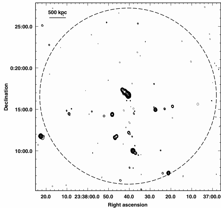
Fig. A.10. GMRT 610 MHz radio contours for the cluster A2631. The 1\sigma level in the image is 80 \mu\text{Jy b}^{-1} . Contours are 0.4 \times (\pm 1, 2, 4, 8, 16\dots) \text{ mJy b}^{-1} . The HPWB is 15'' \times 12'' , PA 0^\circ . The radius of the dashed circle is the virial radius, corresponding to 10.62' for this cluster.
