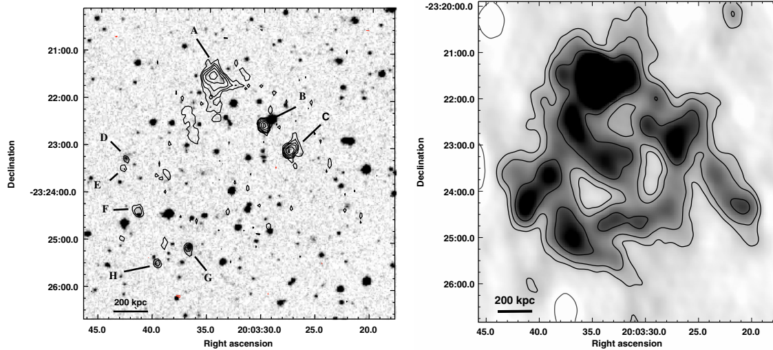
Fig. 6. Left – Full resolution GMRT 610 MHz contours of the central region of RXCJ 2003.5–2323, superposed to the POSS-2 optical image. The resolution of the radio image is 6.9'' \times 5.0'' , PA -0.3^\circ , the 1\sigma level is 40 \mu\text{Jy b}^{-1} . Contours are 0.12 \times (\pm 1, 2, 4, 8\dots) mJy \text{b}^{-1} . Individual sources are labelled from A to H. Right – GMRT 610 MHz gray scale and radio contours of the giant radio halo in RXCJ 2003.5–2323 after subtraction of the individual sources (from B to H in the left panel). The HPWB is 32.0'' \times 23.0'' , PA 15^\circ . Contours are 0.3 \times (\pm 1, 2, 4, 8\dots) mJy \text{b}^{-1} . The 1\sigma level in the image is 100 \mu\text{Jy b}^{-1} .
