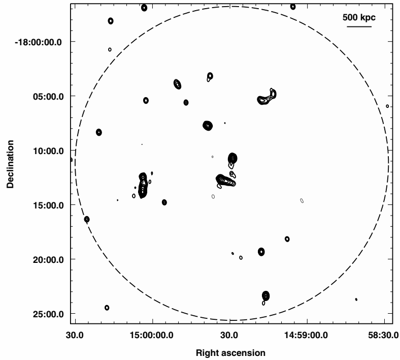
Fig. A.5. GMRT 610 MHz radio contours for the cluster S 780. The 1\sigma level in the image is 65 \mu\text{Jy b}^{-1} . Contours are 0.3 \times (\pm 1, 2, 4, 8, 16\dots) \text{mJy b}^{-1} . The HPWB is 15'' \times 12'' , PA 0^\circ . The radius of the inner circle is the virial radius, corresponding to 14.43' for this cluster.
