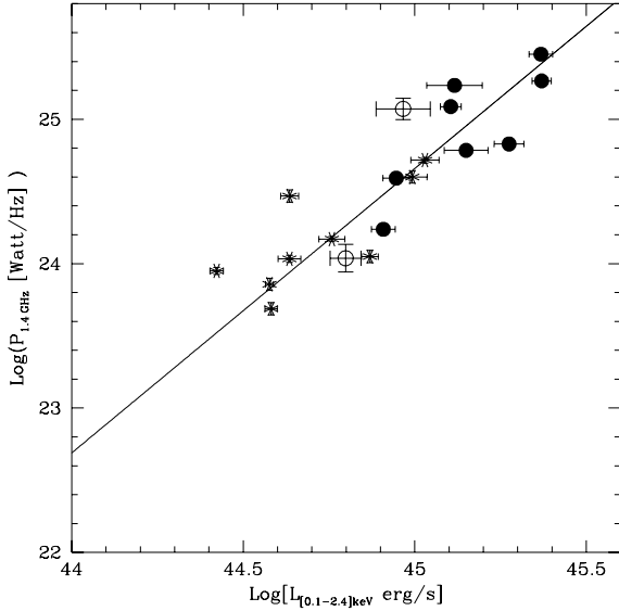
Fig. 10. \text{Log } L_X\text{--}\text{Log } P_{1.4 \text{ GHz}} plot for the clusters with detected giant radio halos. Stars represent the literature clusters at z < 0.2 and filled circles the literature clusters at z > 0.2 . Open circles show the location of A 209 ( lower left ) and RXCJ 2003.5–2323 ( upper right ).
