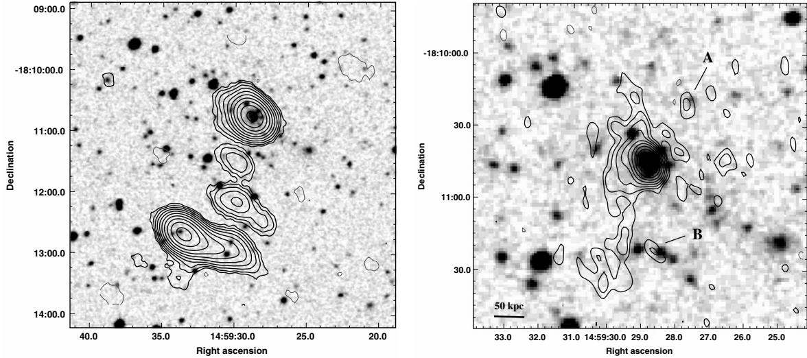
Fig. 9. Left – GMRT 610 MHz radio contours for the cluster S 0780 superposed on the POSS-2 optical plate. The 1\sigma level in the image is 65 \mu\text{Jy b}^{-1} . Contours are 0.20 \times (\pm 1, 2, 4, 8, 16\dots) \text{mJy b}^{-1} . The HPWB is 20.9'' \times 15.9'' , PA 45.9^\circ . Right – High resolution zoom on the central cluster galaxy. The HPWB is 7.5'' \times 5.0'' , PA 25^\circ . Contours are 0.19 \times (\pm 1, 2, 4, 8, 16\dots) \text{mJy b}^{-1} (first contour is 3\sigma ).
