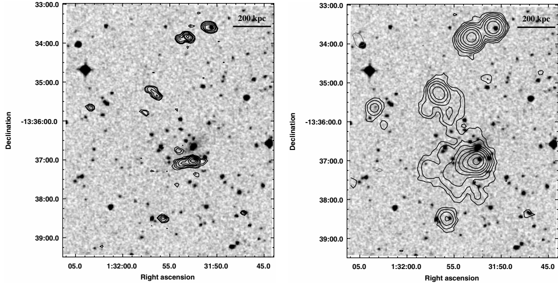
Fig. 2. Left – GMRT 610 MHz radio contours for the A209 cluster superposed on the POSS-2 optical plate. The 1\sigma level in the image is 60 \mu\text{Jy b}^{-1} . Contours are 0.3 \times (\pm 1, 2, 4, 8, 16\dots) \text{mJy b}^{-1} . The HPWB is 8.0'' \times 5.0'' , PA 64^\circ . Right – Natural weighted image of the same sky region at the resolution of 18.0'' \times 17.0'' , PA 0^\circ . The rms ( 1\sigma ) in the image is 60 \mu\text{Jy b}^{-1} , contours are 0.18 \times (\pm 1, 2, 4, 8, 16\dots) \text{mJy b}^{-1} .
