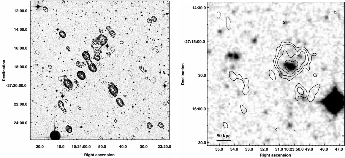
Fig. 8. Left – GMRT 610 MHz radio contours for the cluster A3444 superposed on the POSS-2 optical plate. The 1\sigma level in the image is \sim 50 \mu\text{Jy b}^{-1} . Contours are 0.15 \times (\pm 1, 2, 4, 8, 16\dots) mJy \text{b}^{-1} ( 3\sigma ). The HPWB is 23.2'' \times 16.1'' , PA 37.6^\circ . Right – High resolution zoom on the central cluster galaxy. The HPBW is 7.6'' \times 4.9'' , PA 19^\circ . Contours are given starting from the 3\sigma level: 0.20 \times (\pm 1, 2, 4, 8\dots) .
