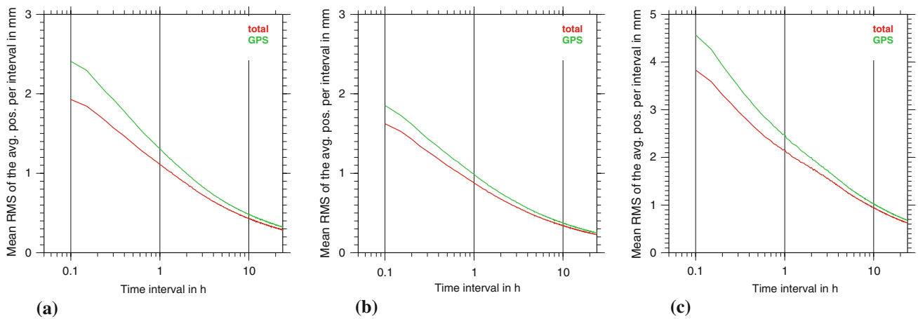
Fig. 12 Standard deviation of the mean position computed over a certain time interval—derived from the kinematic positions (at 3-min intervals over 60 days) of the combined GPS/GLONASS receiver in
