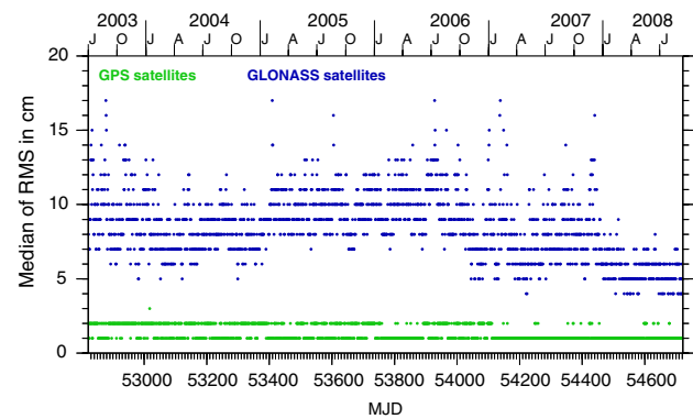
Fig. 6 Median of the RMS for the fit of a 3-day arc through the daily independent orbit solutions for the GPS ( green ) and GLONASS ( blue ) satellites obtained in the combined GPS/GLONASS processing at CODE since 2003
