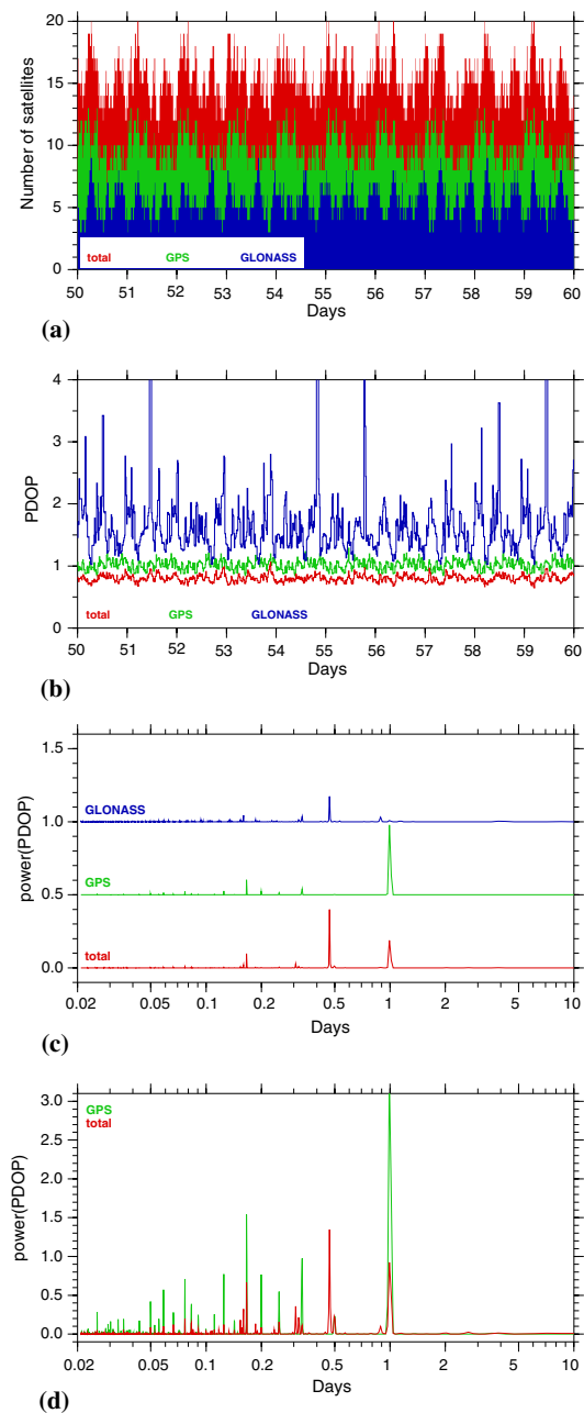
Fig. 10 Comparison of the satellite geometry for IGS station Zimmerwald for the GPS (green), GLONASS (blue), and combined (red) satellite constellation. An elevation cut-off of 5^\circ is assumed. a Number of satellites for station Zimmerwald for 10 days in 2008. b PDOP for station Zimmerwald for 10 days in 2008. c Normalized power spectra of the PDOP time series for station Zimmerwald for 2 months (day 20–79 of year 2008). The three curves are shifted by 0.5 for plotting. d Power spectra of the PDOP time series for station Zimmerwald for 2 months (day 20–79 of year 2008). The curve for the GLONASS-only PDOP values was not plotted because it is much more noisier than the other ones because of the incomplete GLONASS constellation
