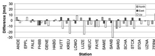
Fig. 15 Discontinuities in the coordinate time series due to the replacement of the antennas at 20 AGNES sites
