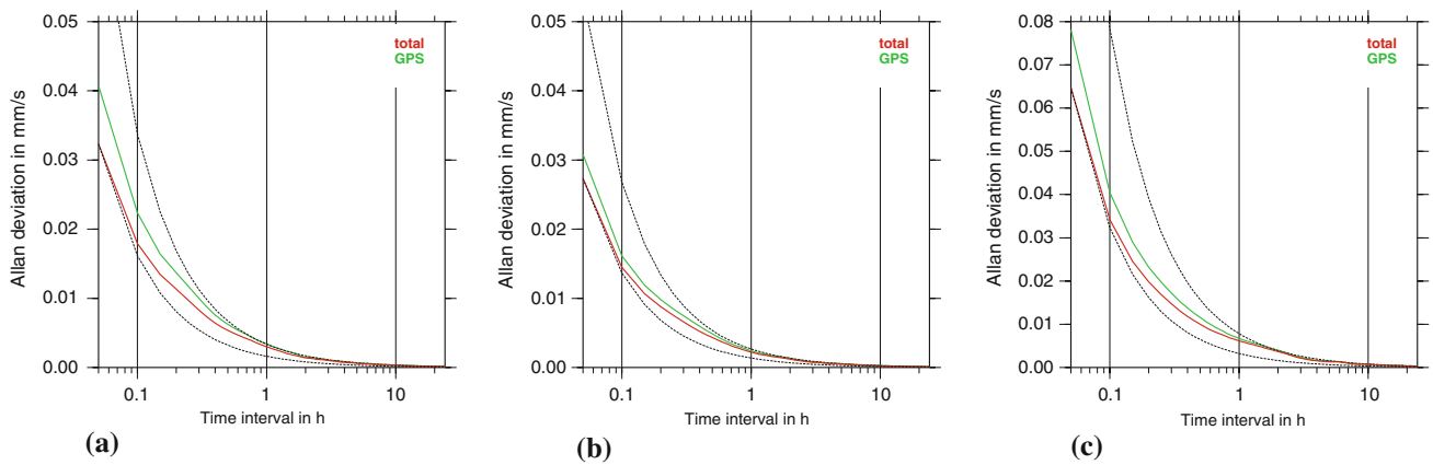
Fig. 11 Allan deviations of the kinematic positions (at 3-min intervals over 60 days) of the combined GPS/GLONASS receiver in Zimmerwald (ZIM2) using only GPS measurements ( green line ) and observations from both GNSS ( red line ), respectively. The unusual non-logarithmic
