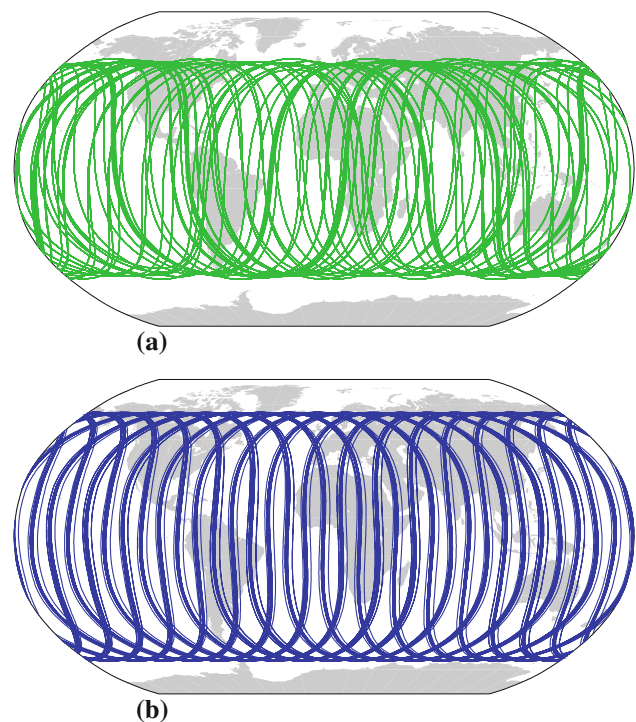
Fig. 8 Ground track of the GPS and GLONASS constellation during 10 days (day 60–69 of year 2008) in February 2008. a Ground track of the GPS satellites. b Ground track of the GLONASS satellites
