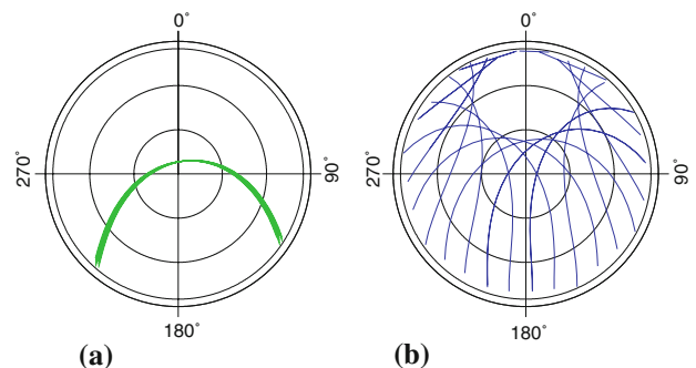
Fig. 9 Elevation-azimuth-diagram for one GPS ( left ) and one GLONASS ( right ) satellite at the location of Zimmerwald, Switzerland, accumulated during 10 days (day 60–69 of year 2008) in February 2008. a GPS satellite G06 b GLONASS satellite R06
