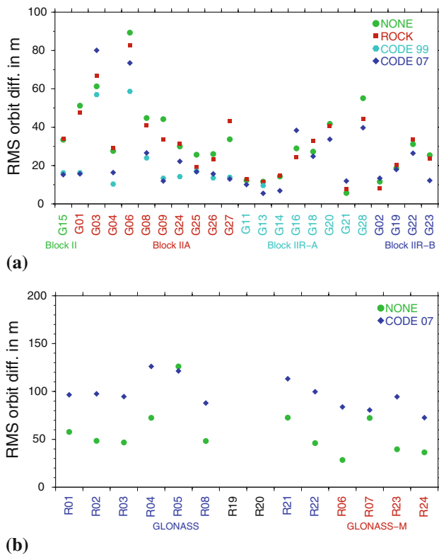
Fig. 3 RMS differences between estimated orbits (“ground truth”) and predicted orbits based on different radiation pressure models. The orbit predictions time span was 2 weeks. Eclipsing satellites are excluded from the differences. a GPS satellites. b GLONASS satellites
