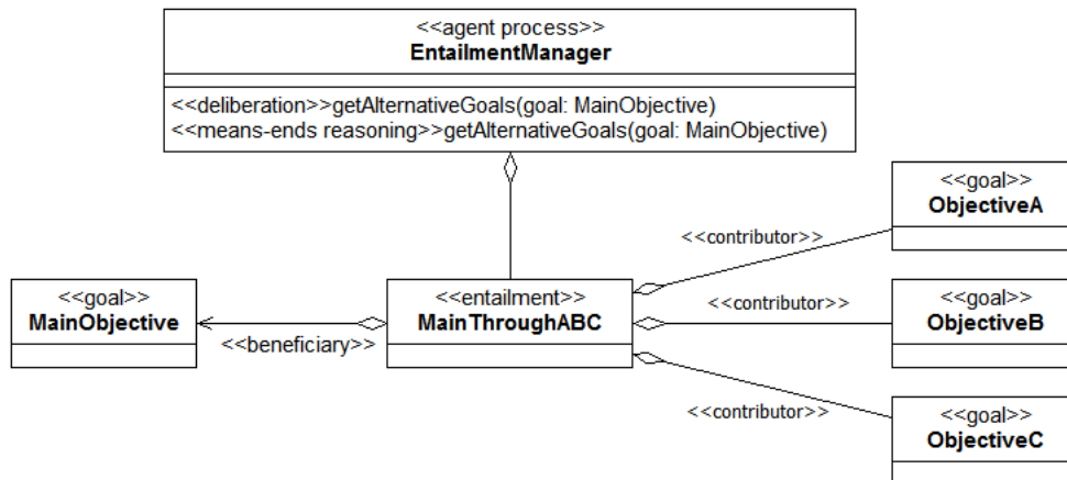
Figure 3: The structure of the Intention Decomposition pattern.
