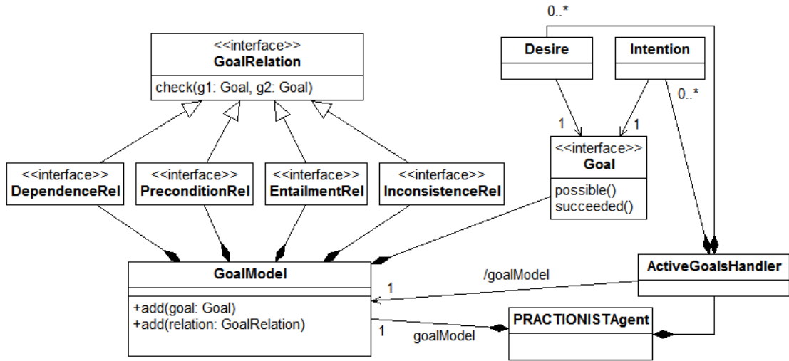
Figure 4: The structure of the support for the goal model in the PRACTIONIST framework.
