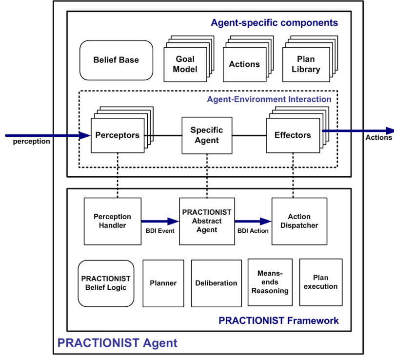
Figure 1: PRACTIONIST Agent Architecture.
