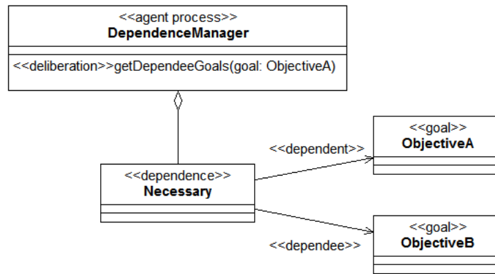
Figure 6: The structure of the Necessary Intention pattern.
