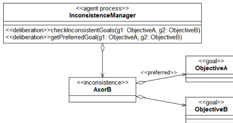
Figure 5: The structure of the Mutually Exclusive Intentions pattern.
