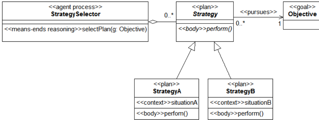
Figure 2: The structure of the Dynamic Strategy Selection pattern.
