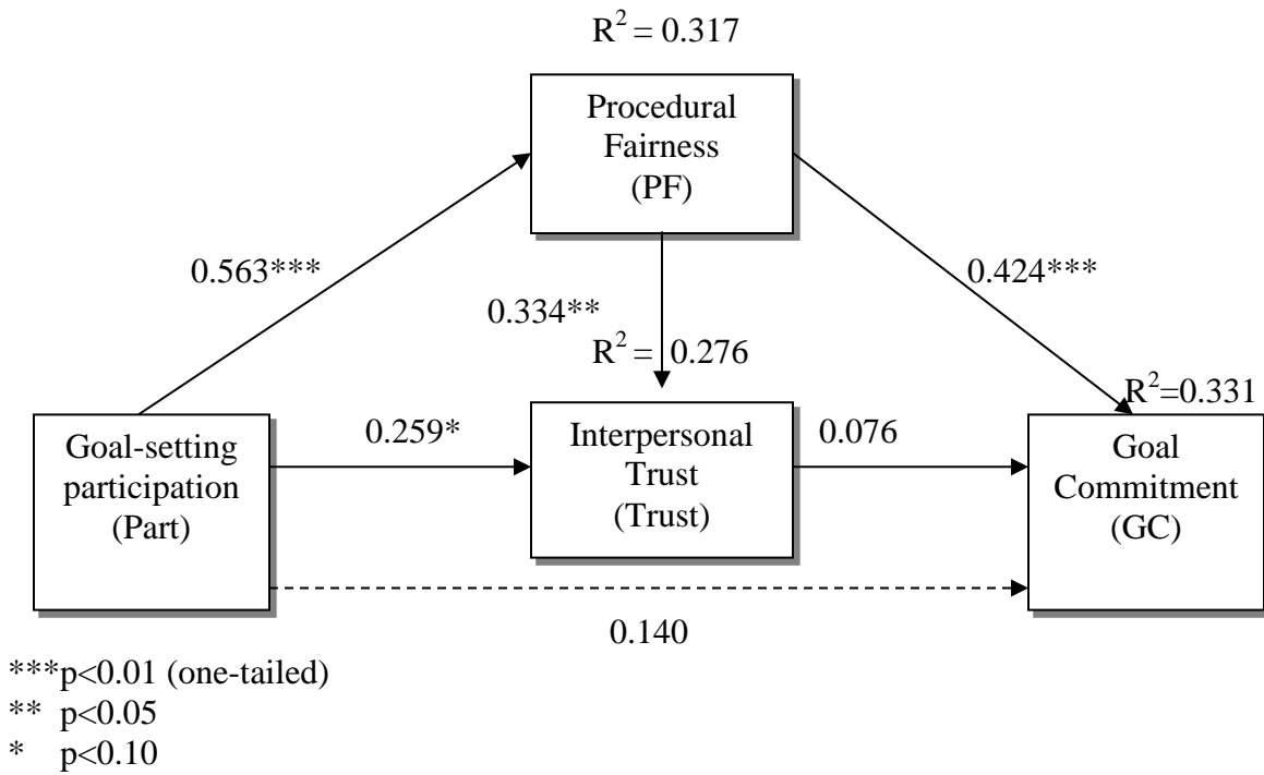
Figure 2. PLS Results
