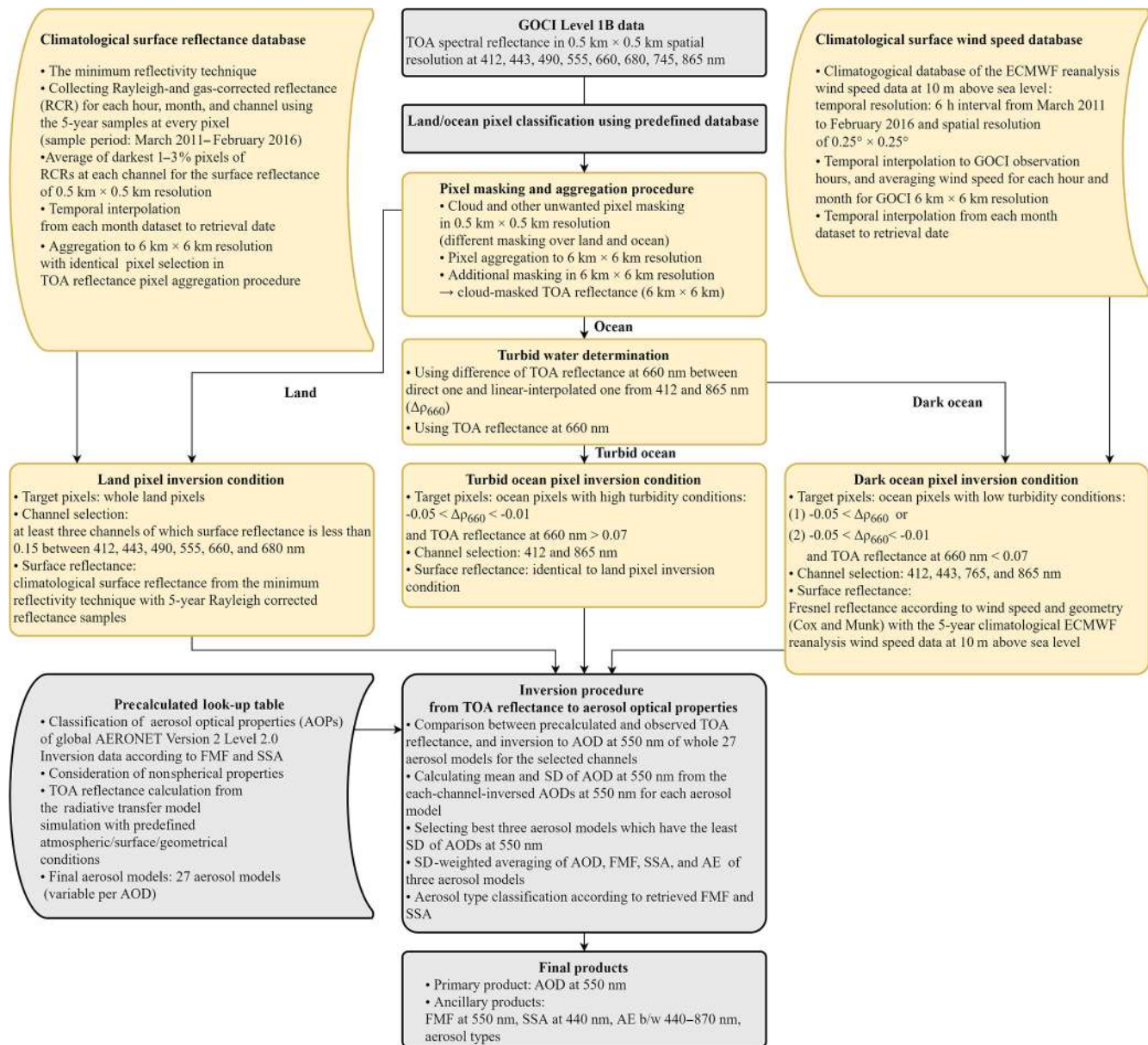
Figure 1. Flow chart of the GOCI Yonsei aerosol retrieval version 2 algorithm. Yellow indicates improvements from version 1 to version 2, and grey indicates no change from version 1.
