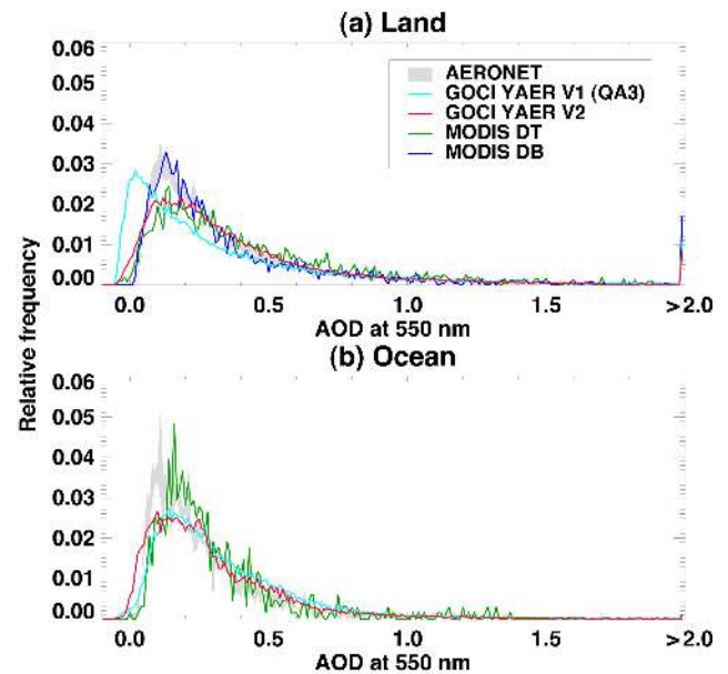
Figure 4. Relative frequency histograms of retrieved AOD from AERONET and satellites over (a) land and (b) ocean surfaces.
