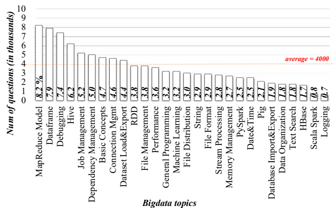
Figure 2: Big data topics and number of their questions.
