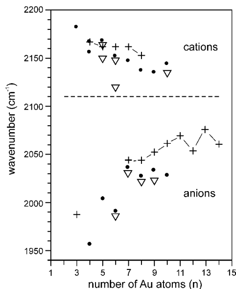
Figure 4. Comparison of the values of \nu(\text{CO}) for anionic and cationic gold cluster carbonyls, \text{Au}_n(\text{CO})_m^- , as a function of cluster size, n , and CO uptake, m . The monocarbonyl complexes ( m = 1 ) are represented by joined + symbols and the saturated complexes by solid circles. The saturated stoichiometries, as given by (n, m) , are (4,4), (5,4), (6,6), (7,4), (8,4), (9,6), and (10,6) for the anions and (3,3), (4,4), (5,4), (6,5), (7,6), (8,7), (9,8), and (10,6) for the cations. In the cases of intermediate saturation the higher complexes formed at high p(\text{CO}) are represented by open triangles ( \nabla ). For complexes with several absorption features, all values are depicted. The absolute uncertainties of the values are typically \pm 10\text{ cm}^{-1} , but relative shifts can be determined more precisely. The dashed line indicates the \nu(\text{CO}) value for CO adsorbed on gold surfaces.
